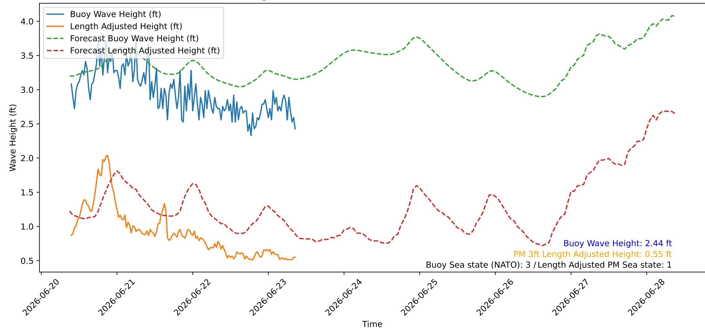
Wave Heights over Time for Red Beach at 2026-06-23 09:20:46
