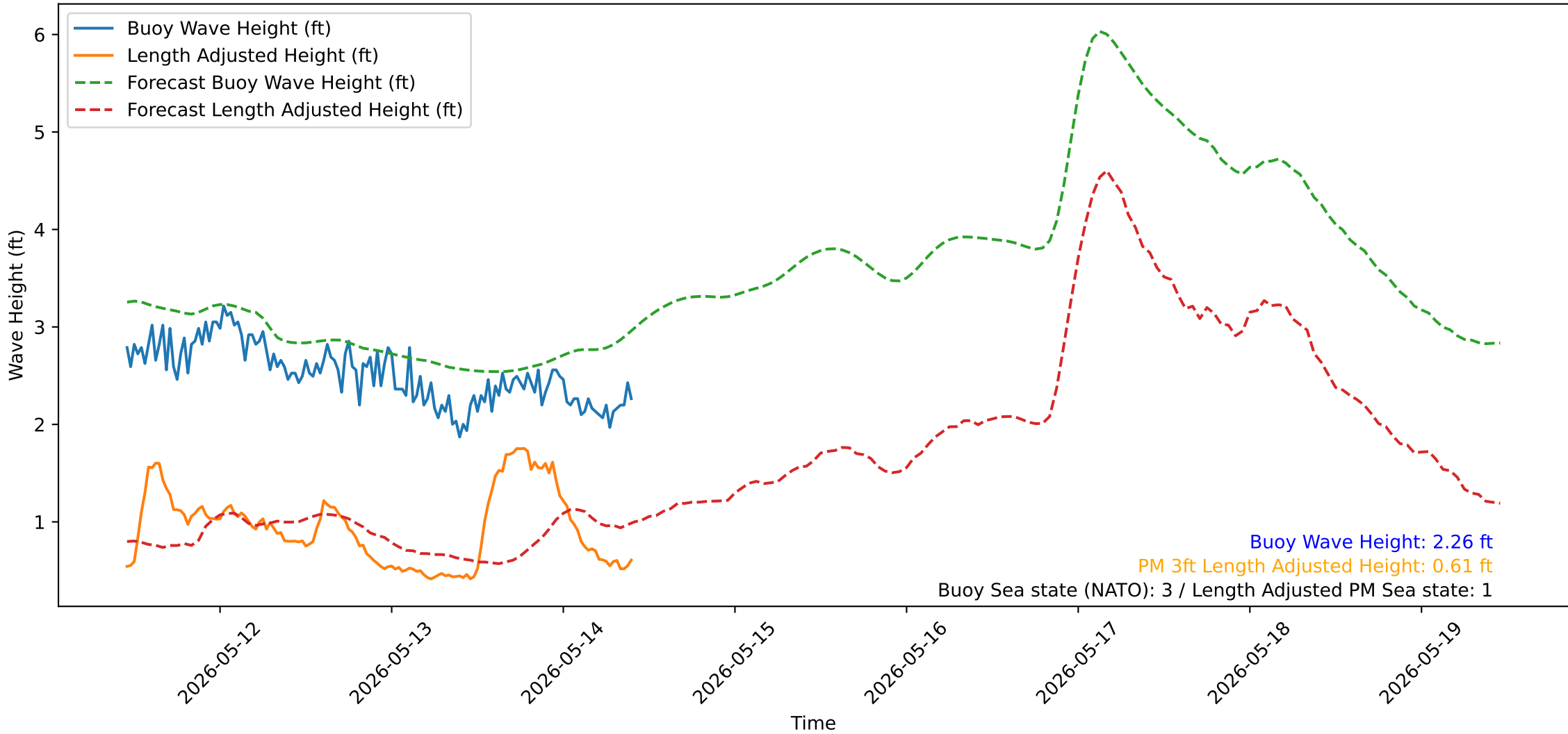
Wave Heights over Time for Red Beach at 2026-05-14 10:30:51
