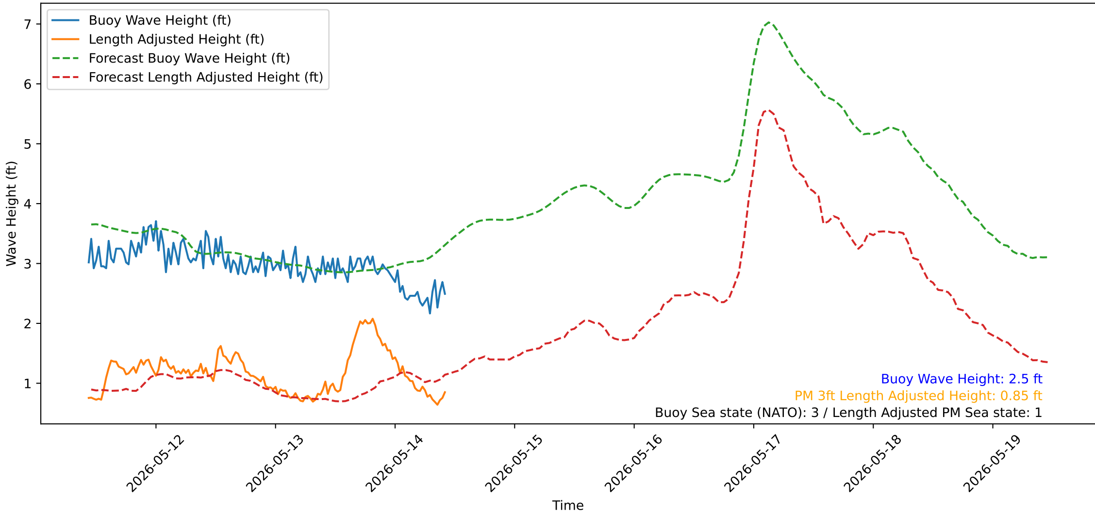
Wave Heights over Time for Oceanside Harbor at 2026-05-14 10:30:32
