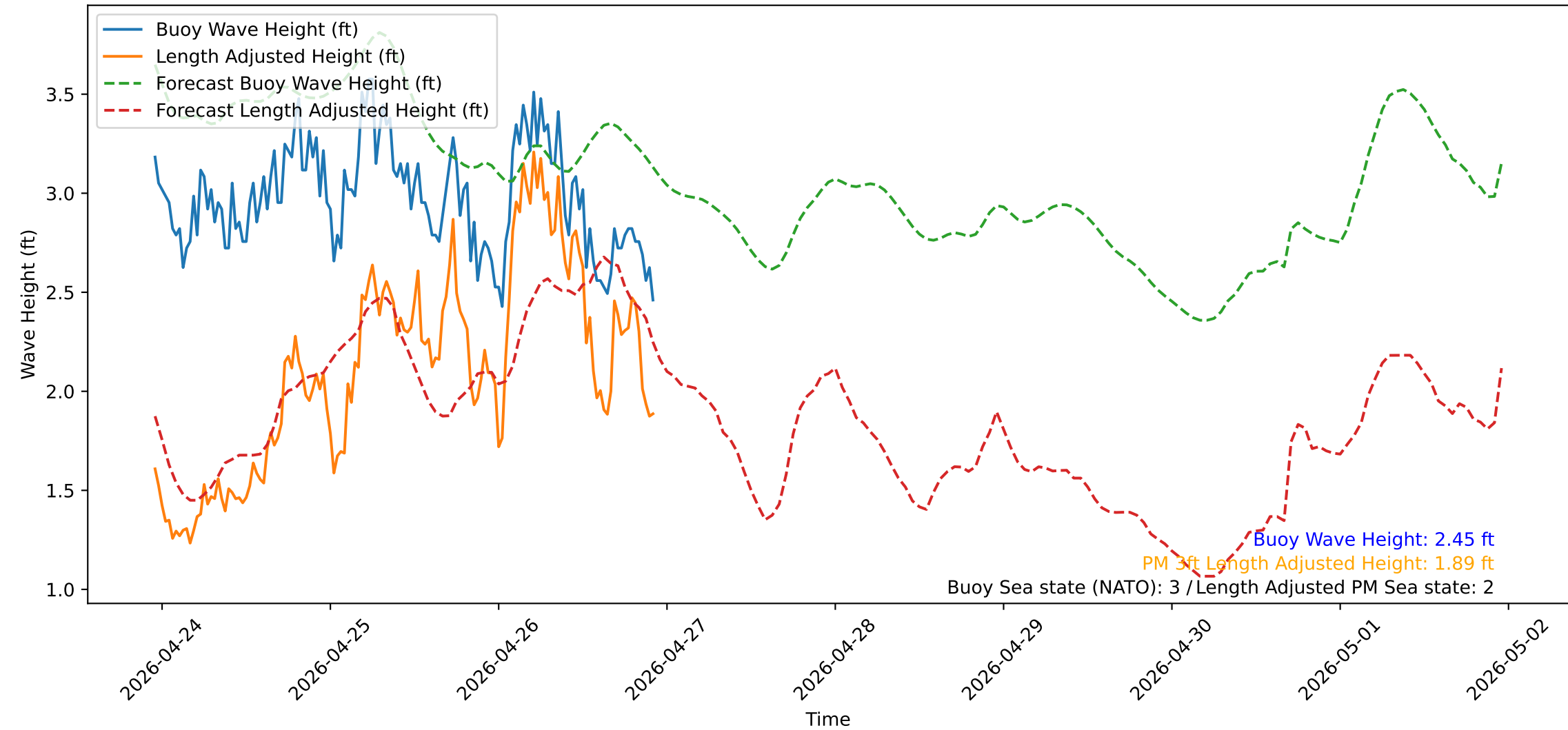
Wave Heights over Time for Green Beach at 2026-04-26 23:01:13
