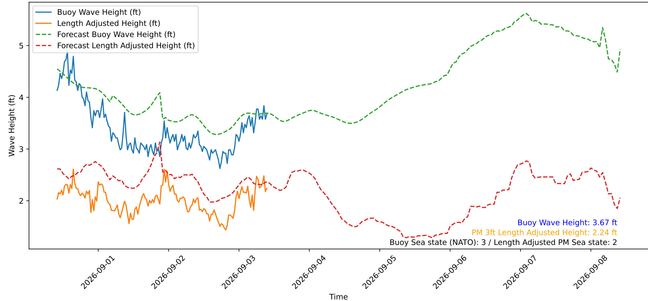
Wave Heights over Time for Oceanside Harbor at 2026-09-03 10:10:30
