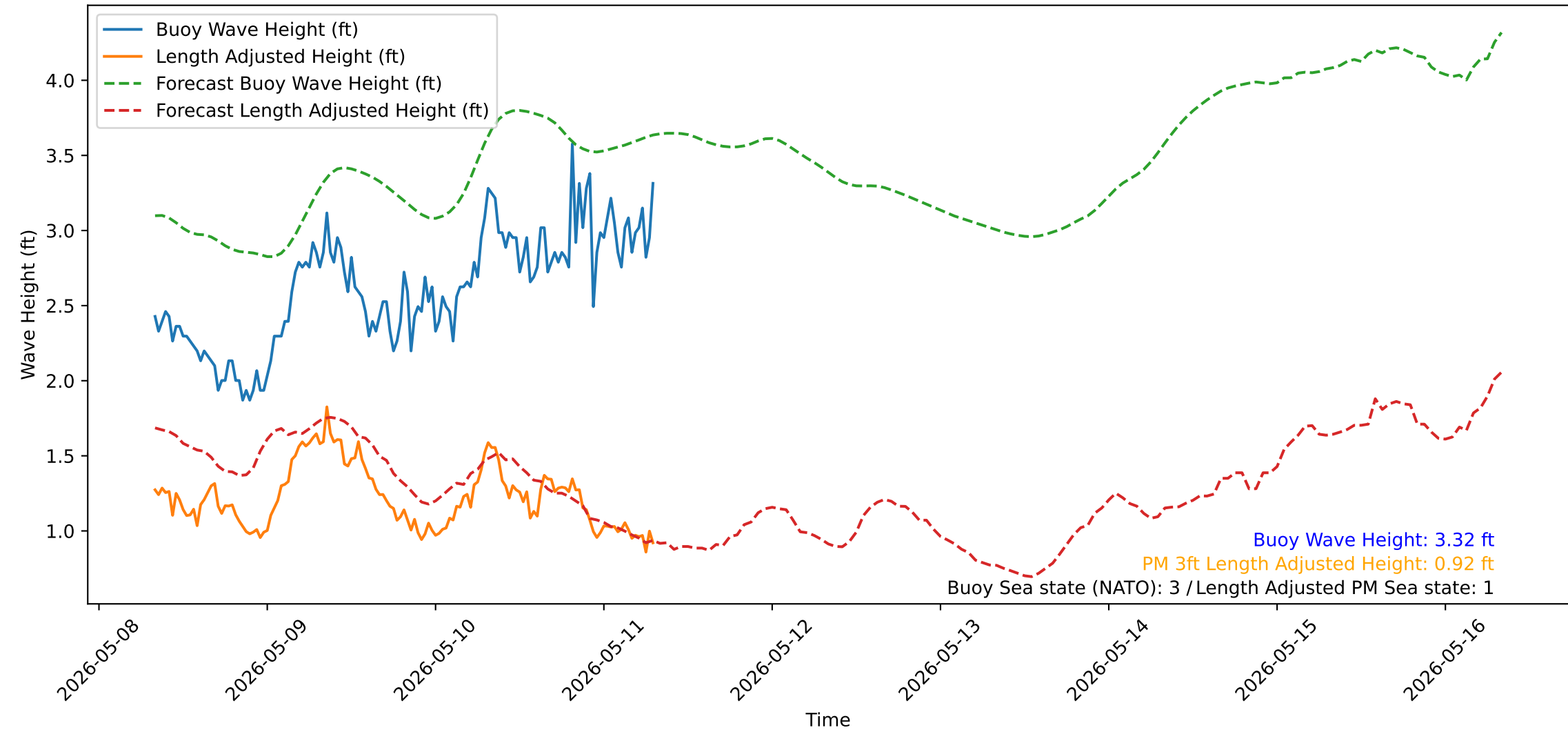
Wave Heights over Time for Oceanside Harbor at 2026-05-11 08:00:32
