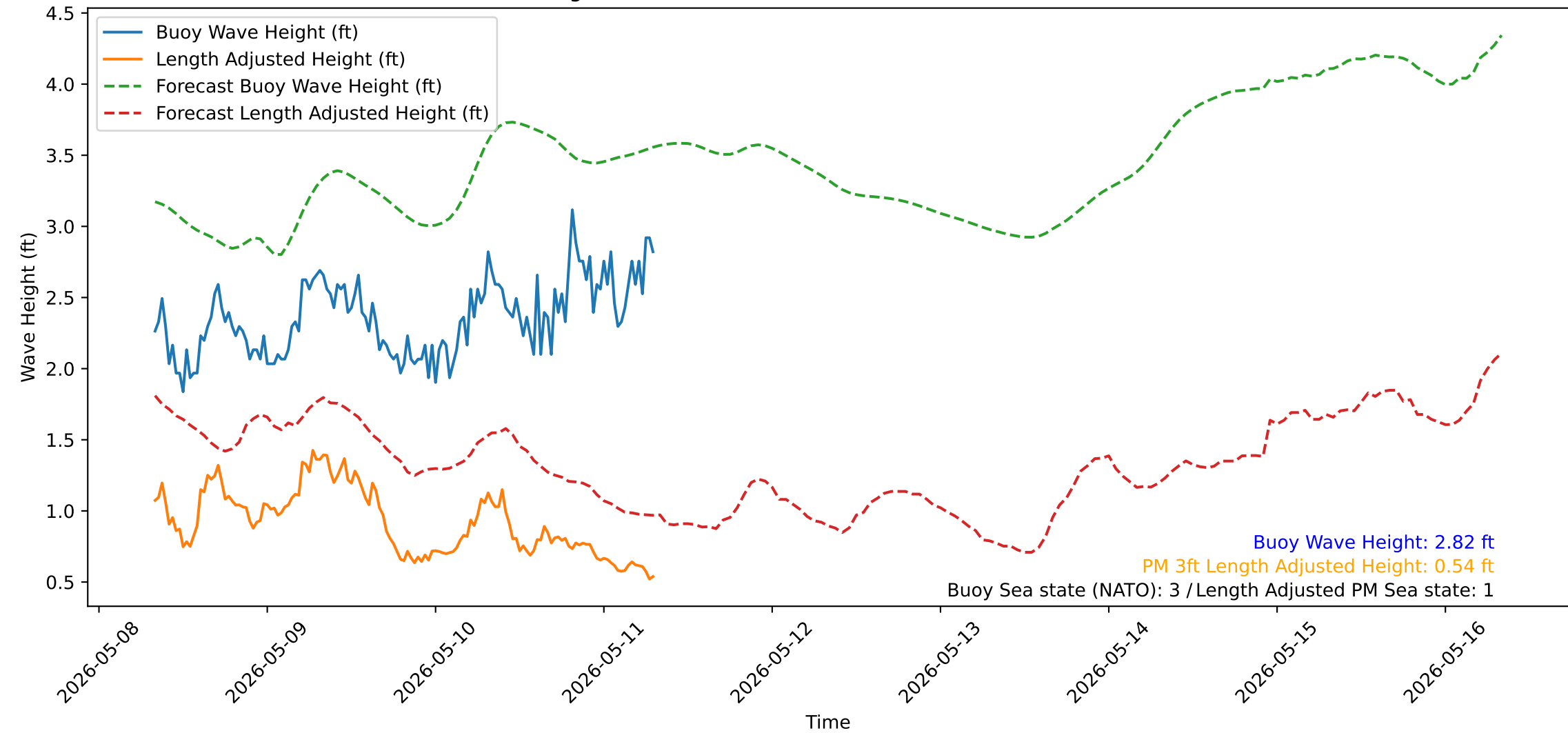
Wave Heights over Time for Green Beach at 2026-05-11 08:01:13
