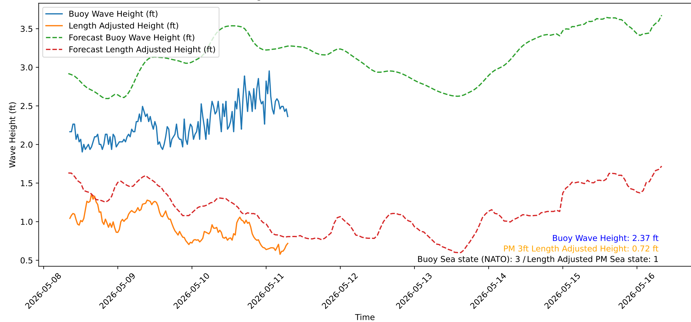
Wave Heights over Time for Red Beach at 2026-05-11 08:00:51
