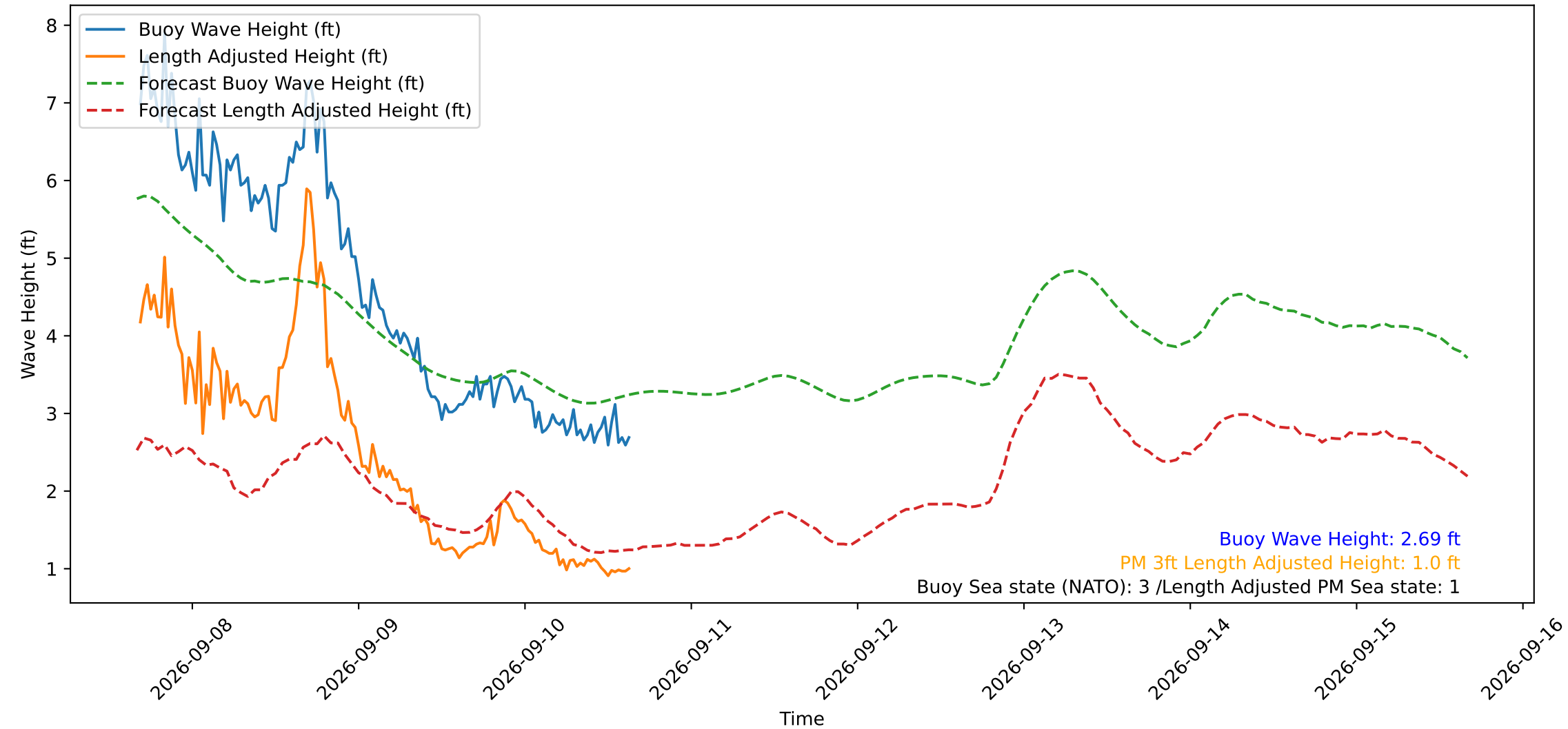
Wave Heights over Time for Green Beach at 2026-09-10 16:01:12
