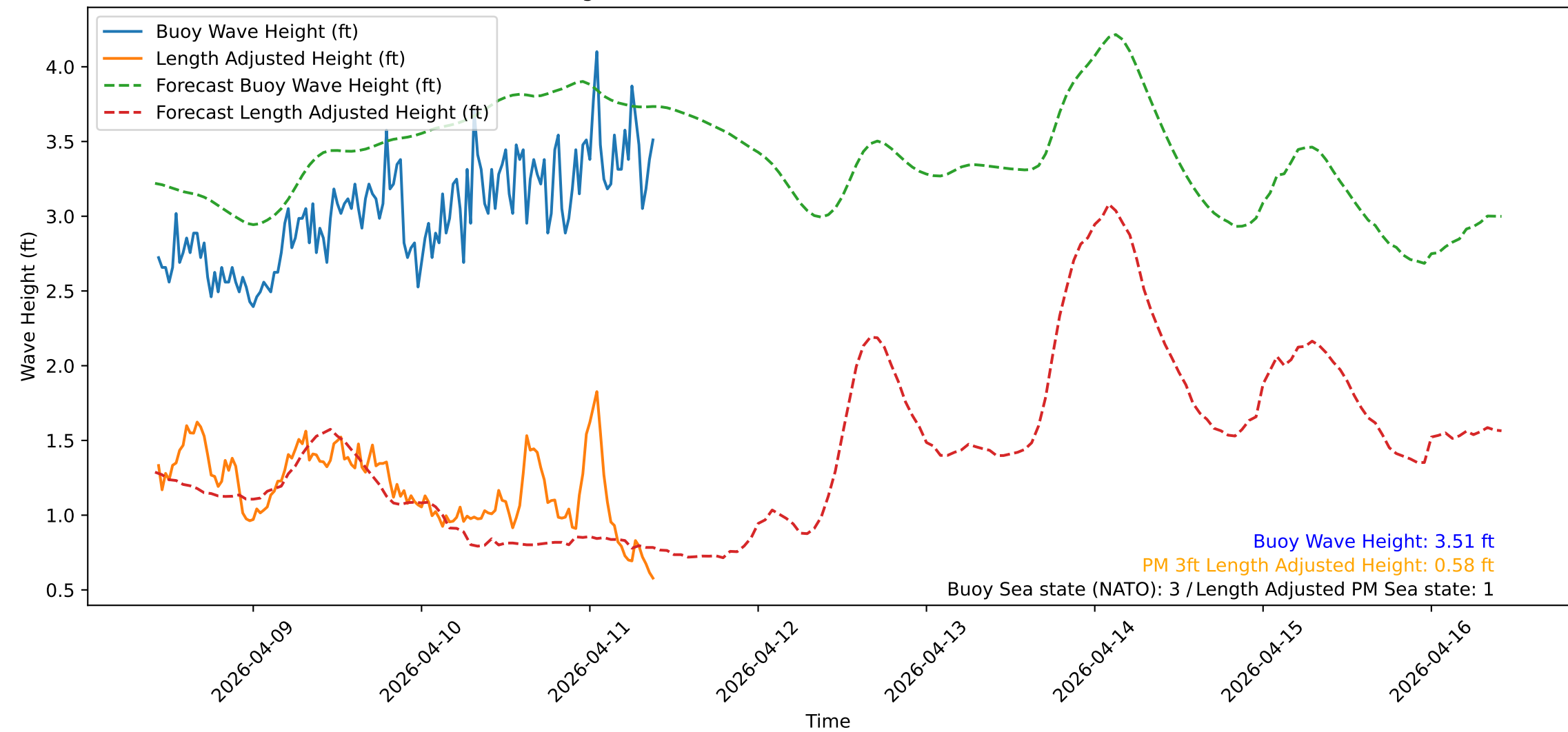
Wave Heights over Time for Red Beach at 2026-04-11 10:00:51
