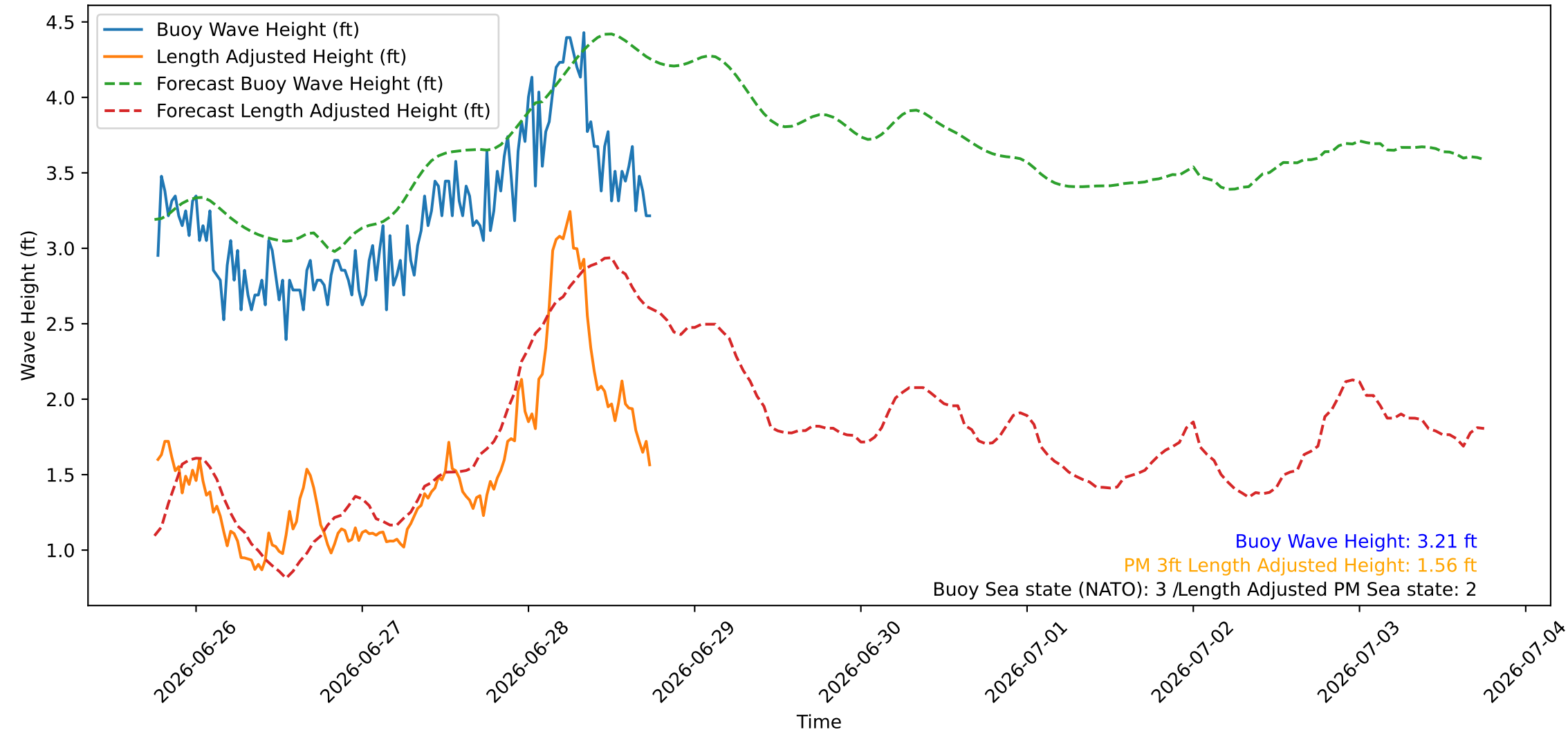
Wave Heights over Time for Oceanside Harbor at 2026-06-28 18:20:26
