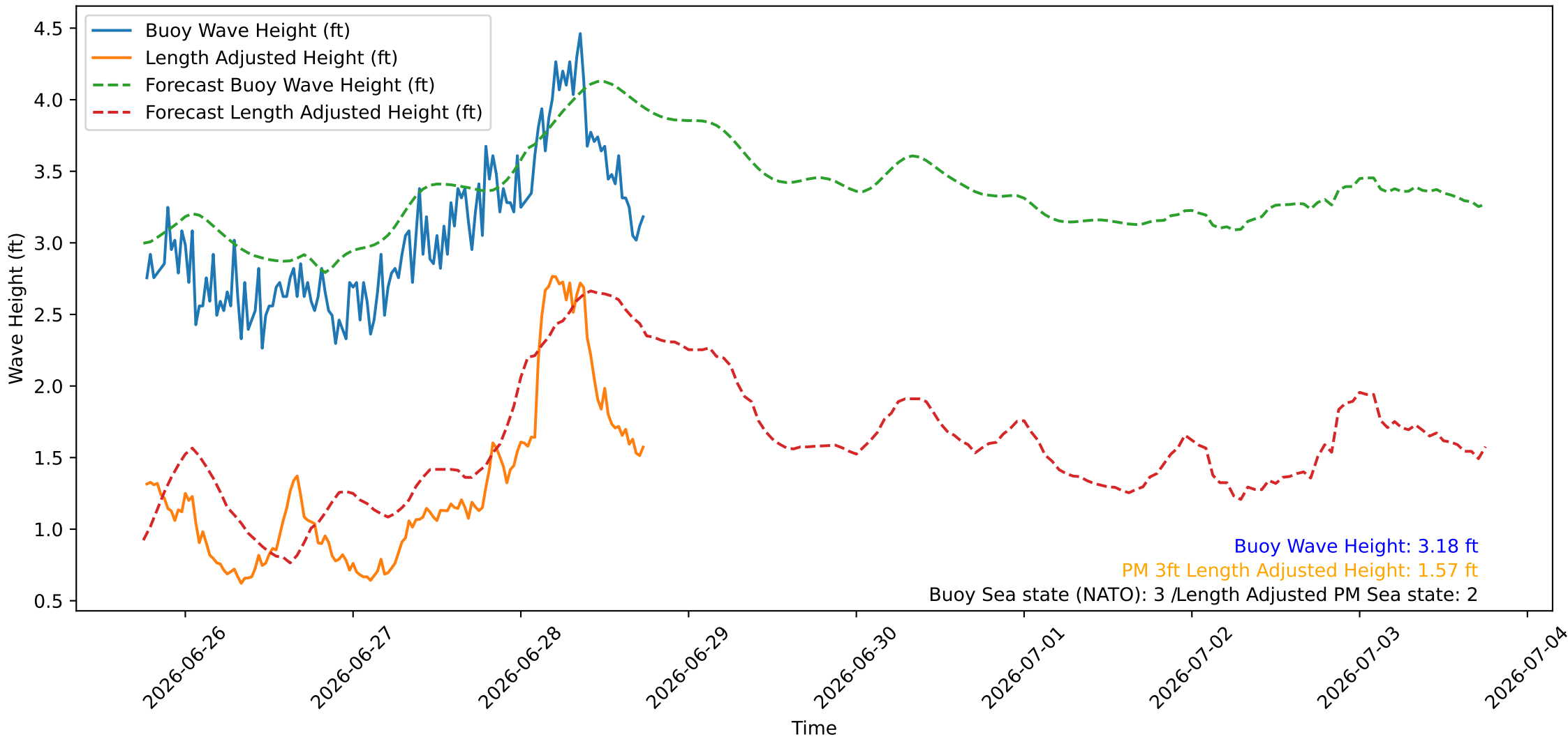
Wave Heights over Time for Red Beach at 2026-06-28 18:20:47
