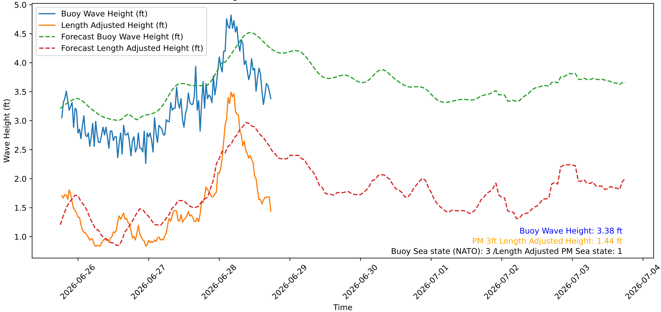
Wave Heights over Time for Green Beach at 2026-06-28 18:21:09
