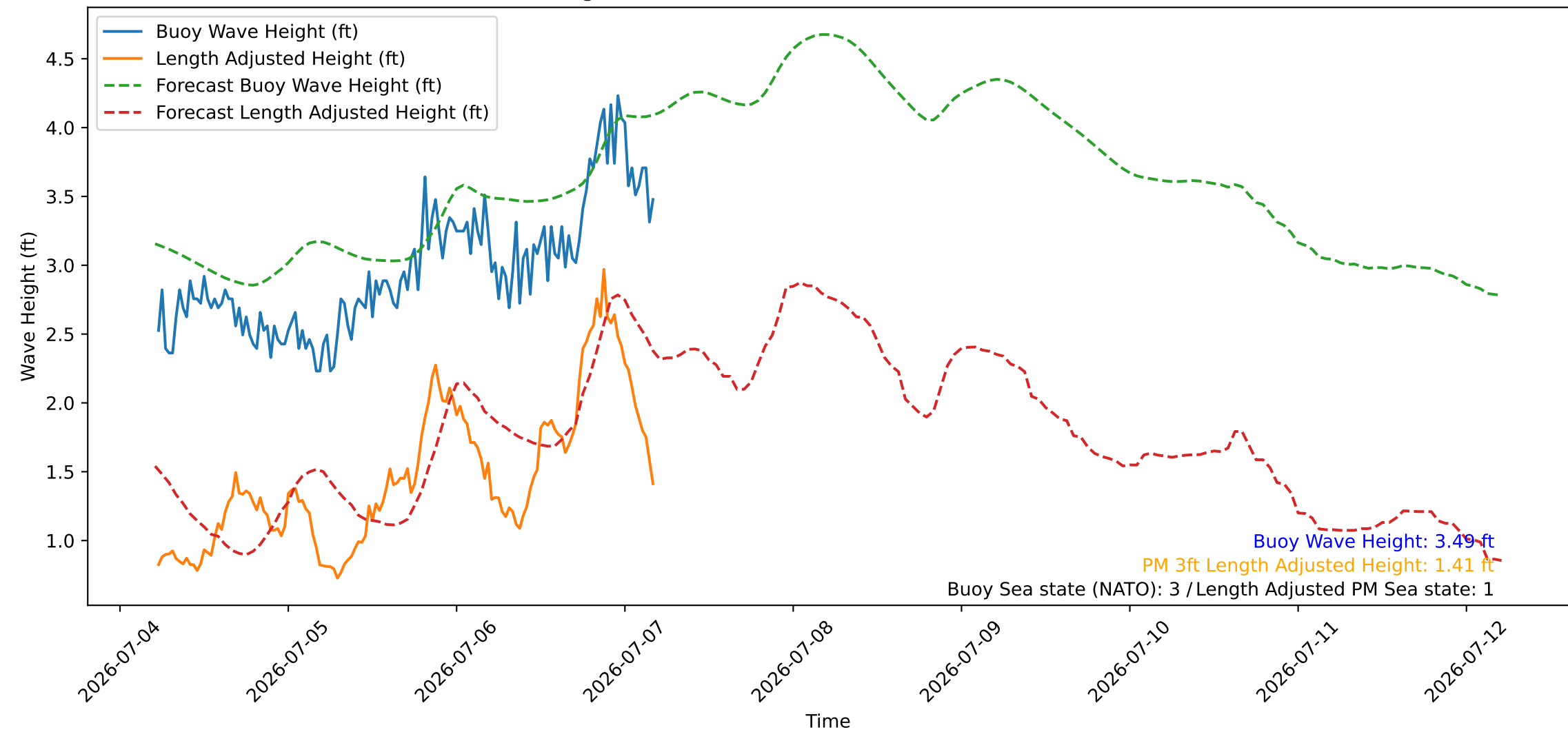
Wave Heights over Time for Red Beach at 2026-07-07 05:00:46
