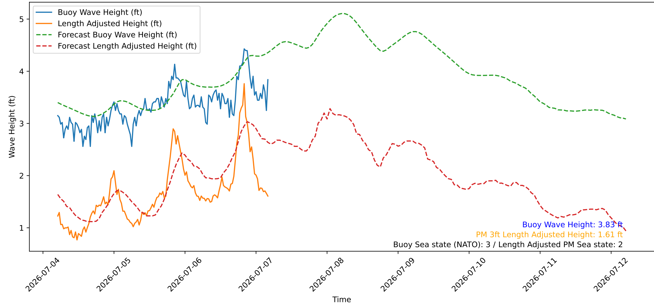
Wave Heights over Time for Green Beach at 2026-07-07 05:01:09
