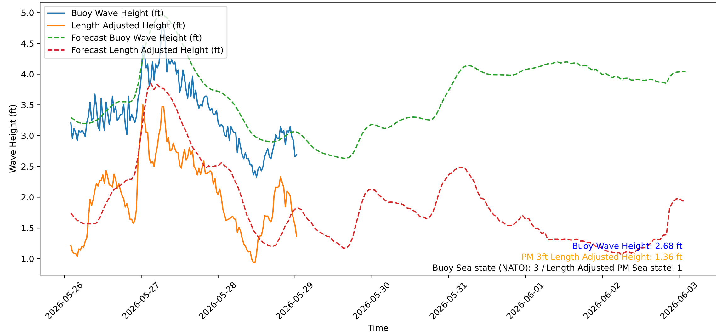
Wave Heights over Time for Red Beach at 2026-05-29 01:30:50
