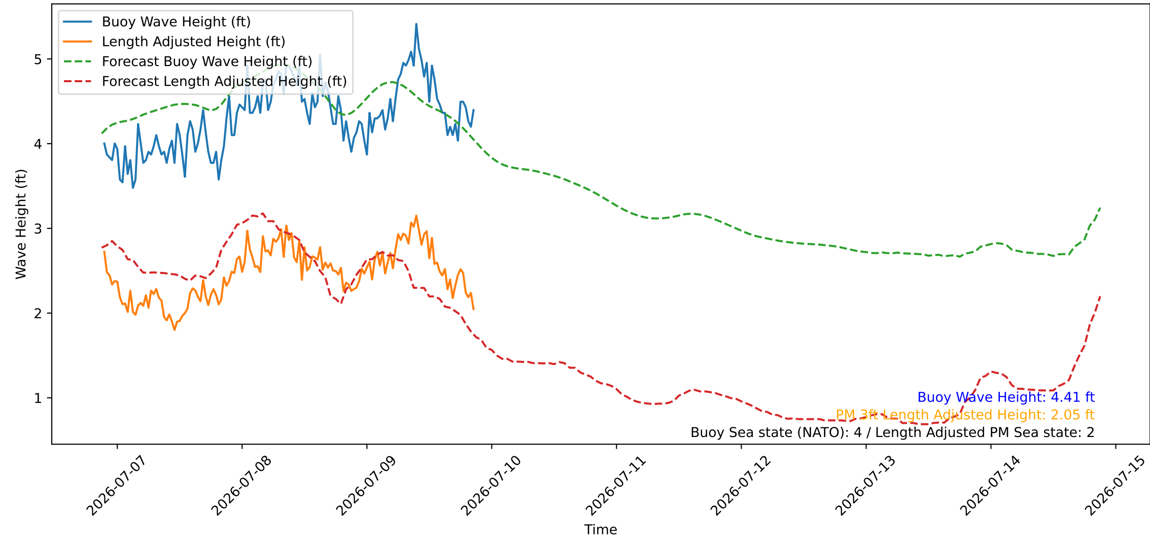
Wave Heights over Time for Oceanside Harbor at 2026-07-09 21:20:26
