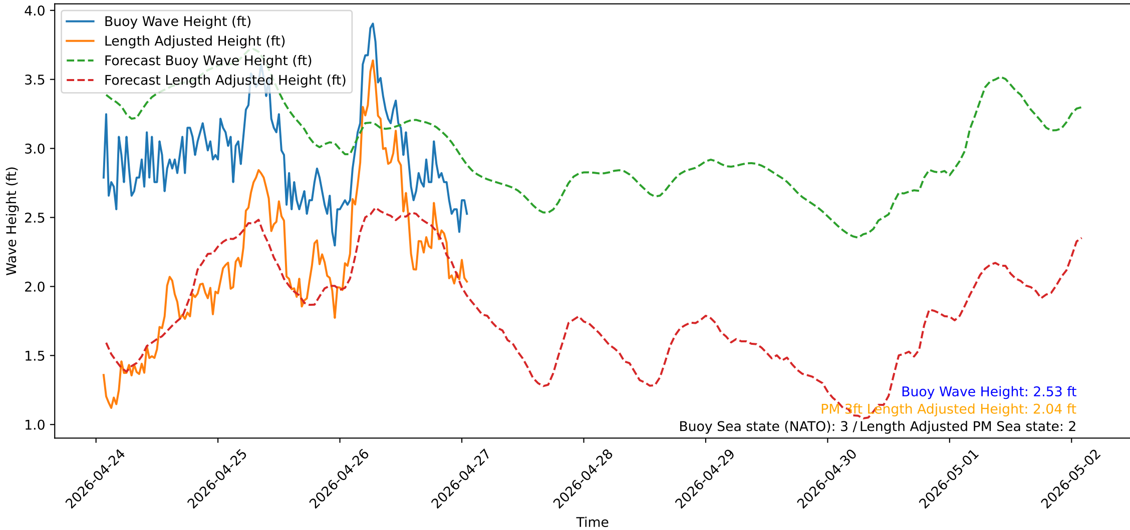
Wave Heights over Time for Oceanside Harbor at 2026-04-27 01:30:31
