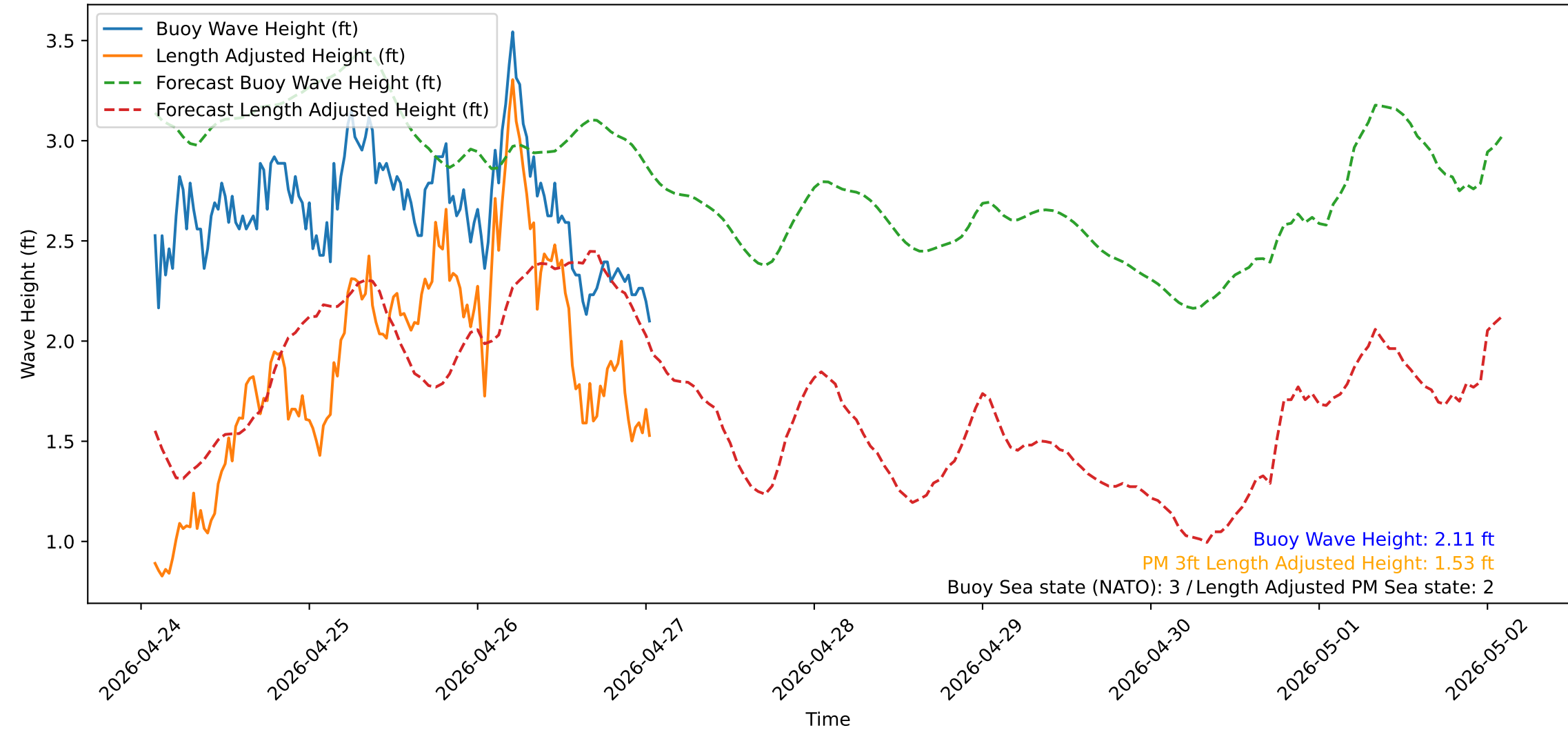
Wave Heights over Time for Red Beach at 2026-04-27 01:30:51
