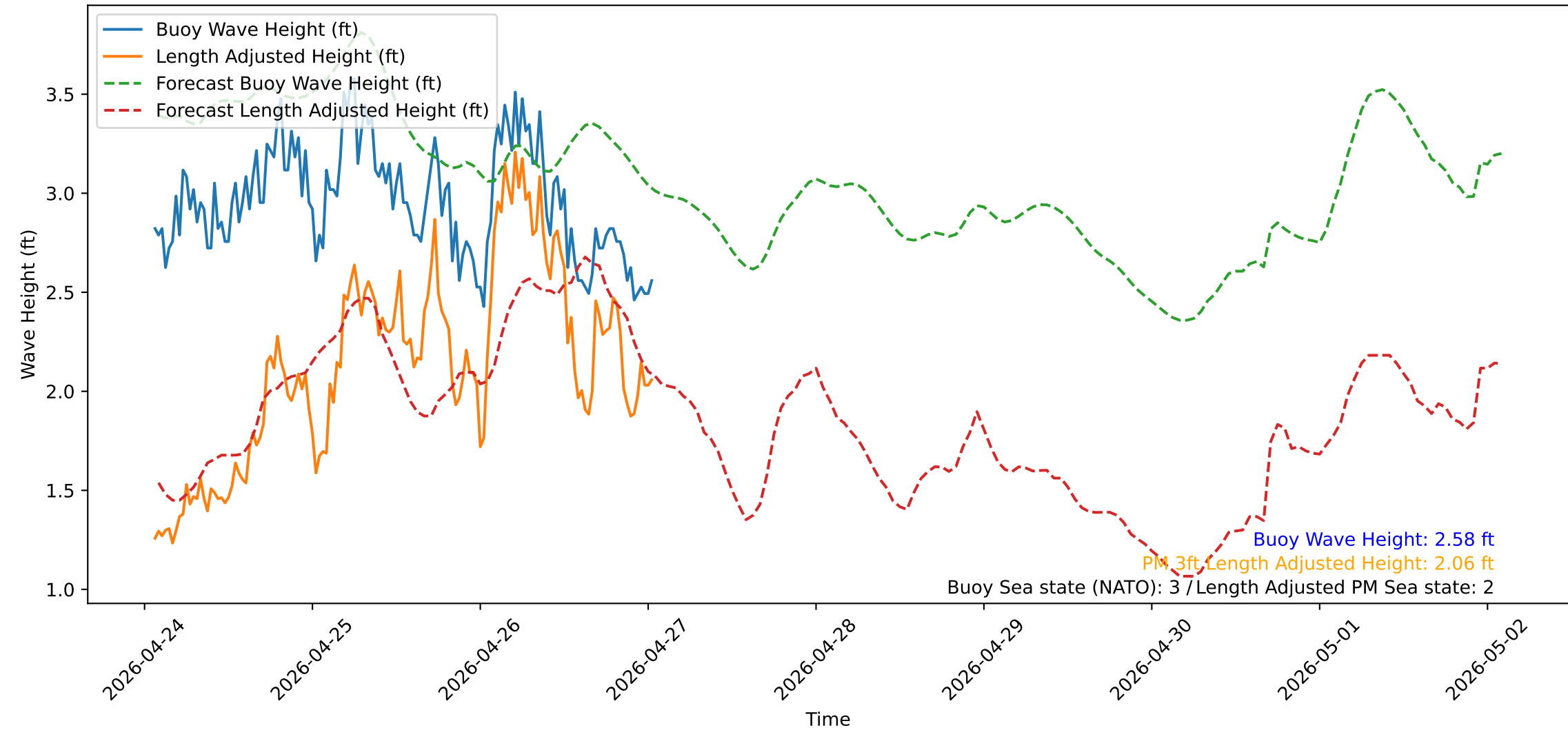
Wave Heights over Time for Green Beach at 2026-04-27 01:31:13
