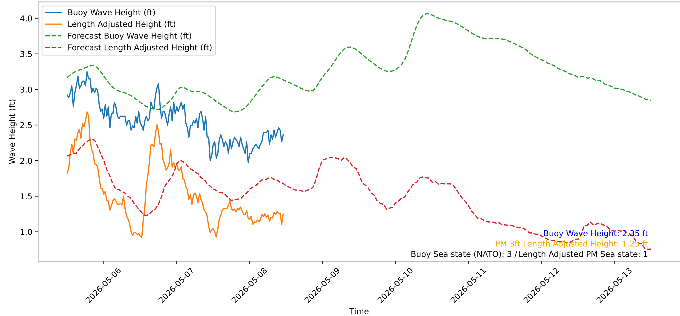
Wave Heights over Time for Oceanside Harbor at 2026-05-08 11:50:31
