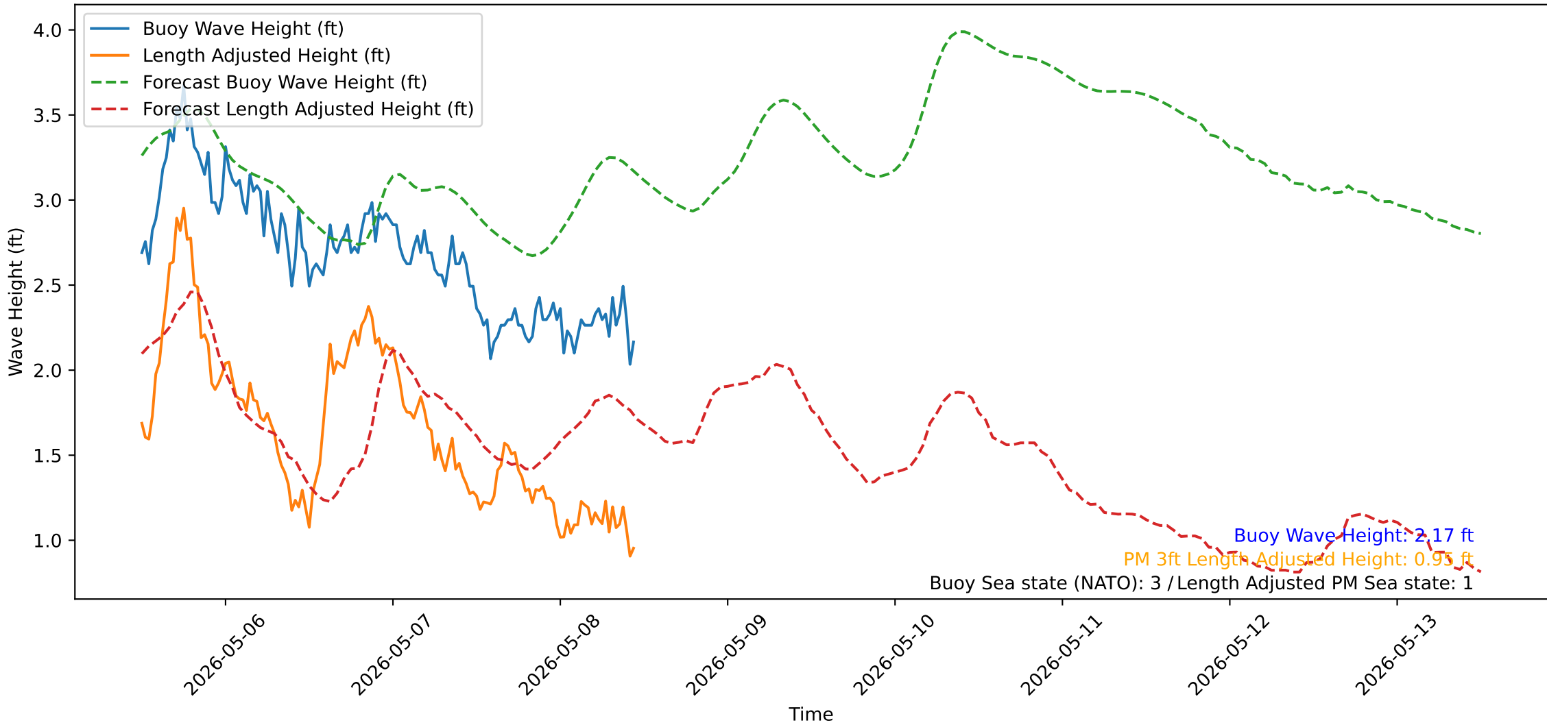
Wave Heights over Time for Green Beach at 2026-05-08 11:51:15
