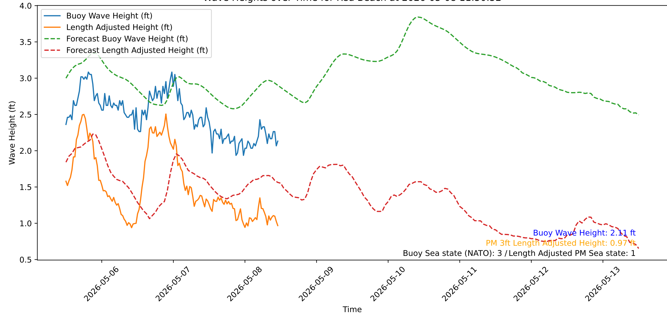
Wave Heights over Time for Red Beach at 2026-05-08 11:50:52
