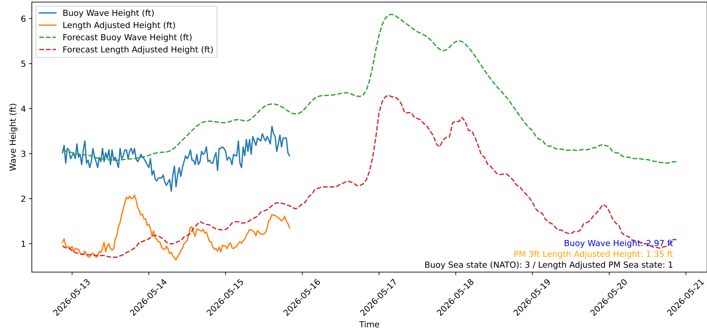
Wave Heights over Time for Oceanside Harbor at 2026-05-15 20:50:31
