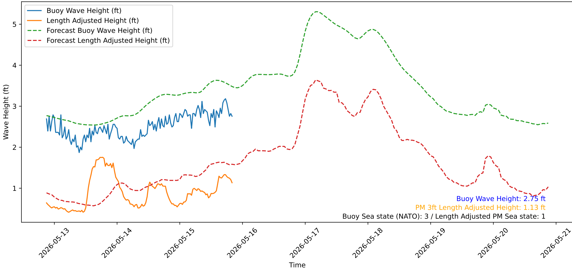
Wave Heights over Time for Red Beach at 2026-05-15 20:50:51
