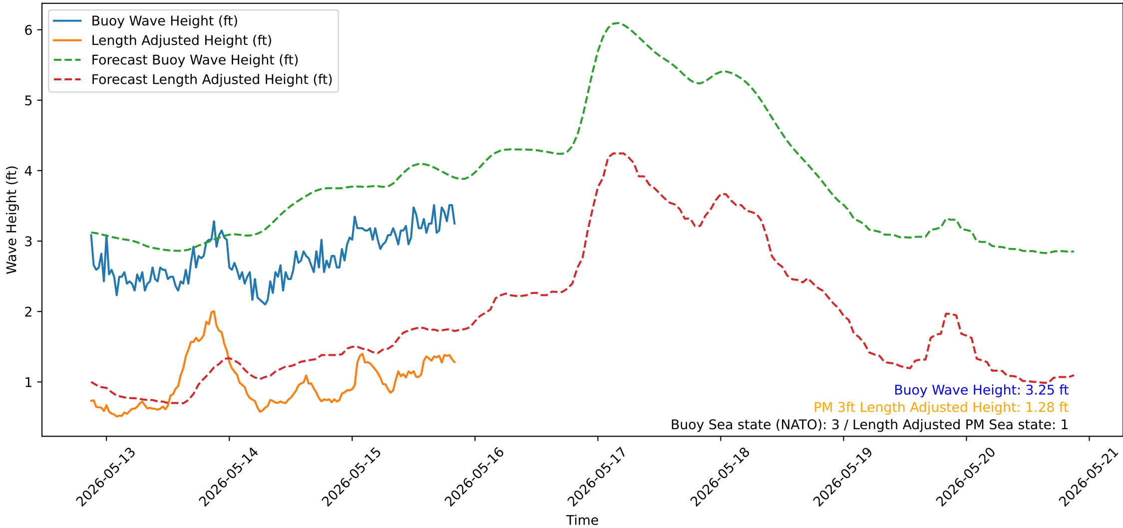
Wave Heights over Time for Green Beach at 2026-05-15 20:51:14
