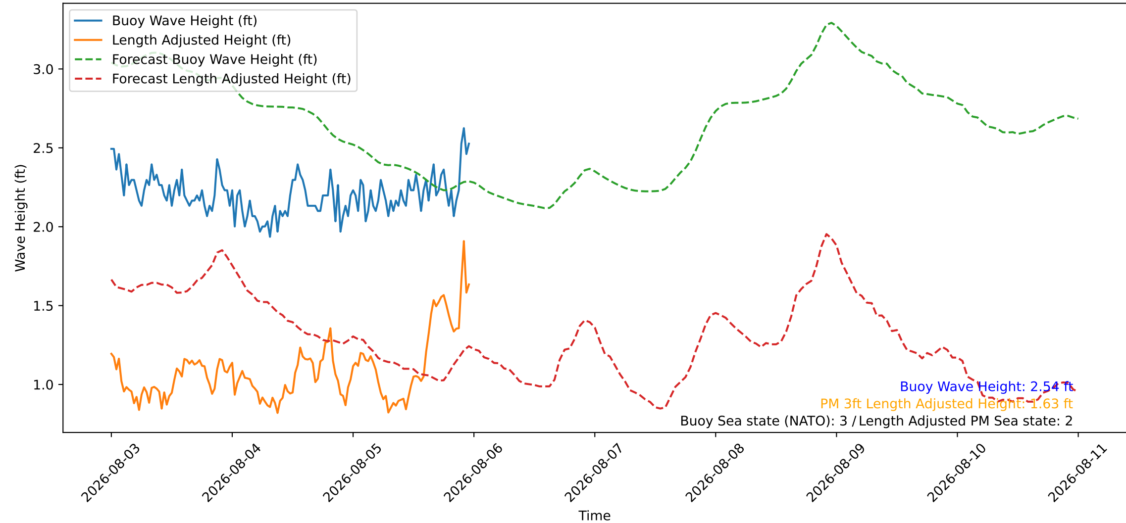
Wave Heights over Time for Green Beach at 2026-08-06 00:01:07
