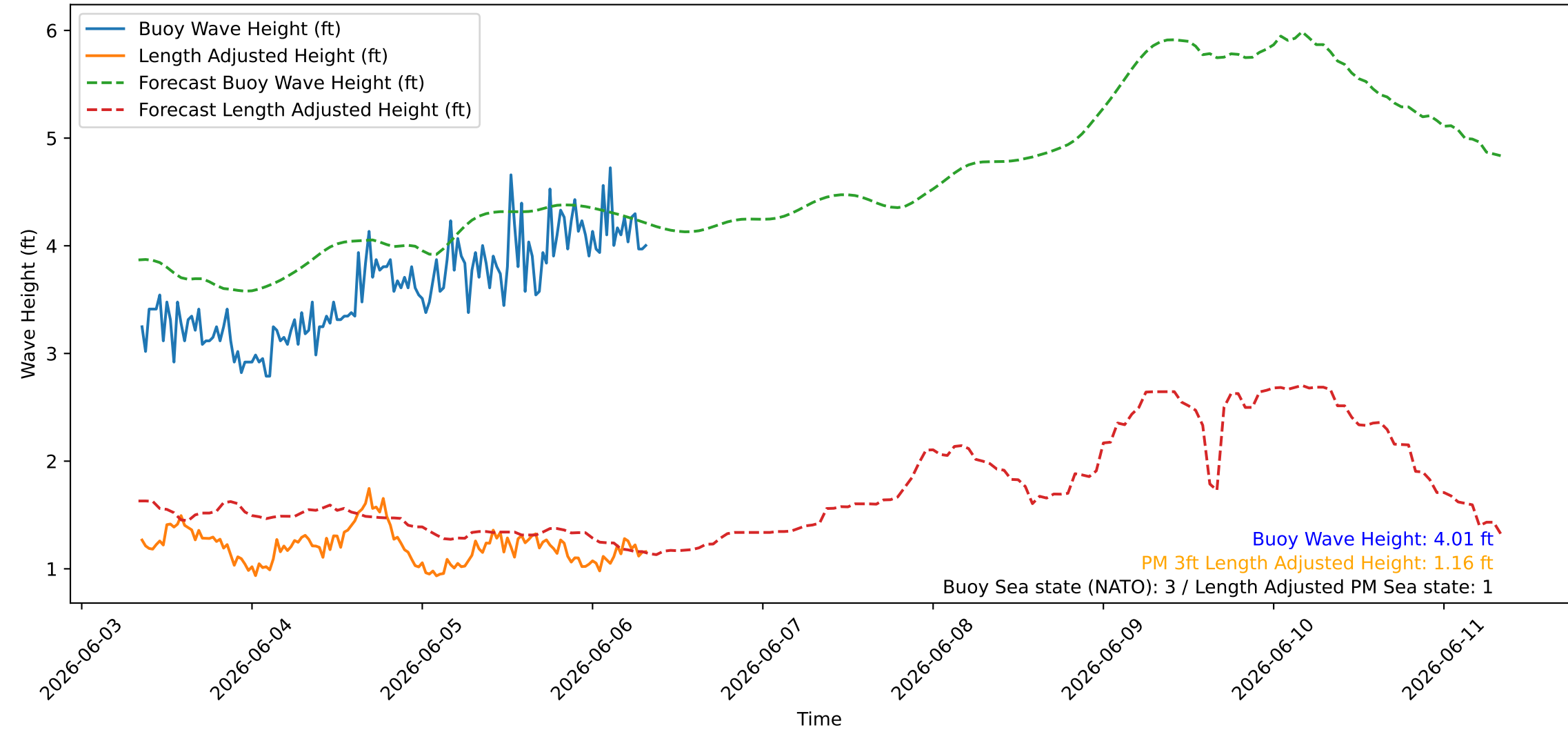
Wave Heights over Time for Green Beach at 2026-06-06 08:21:09
