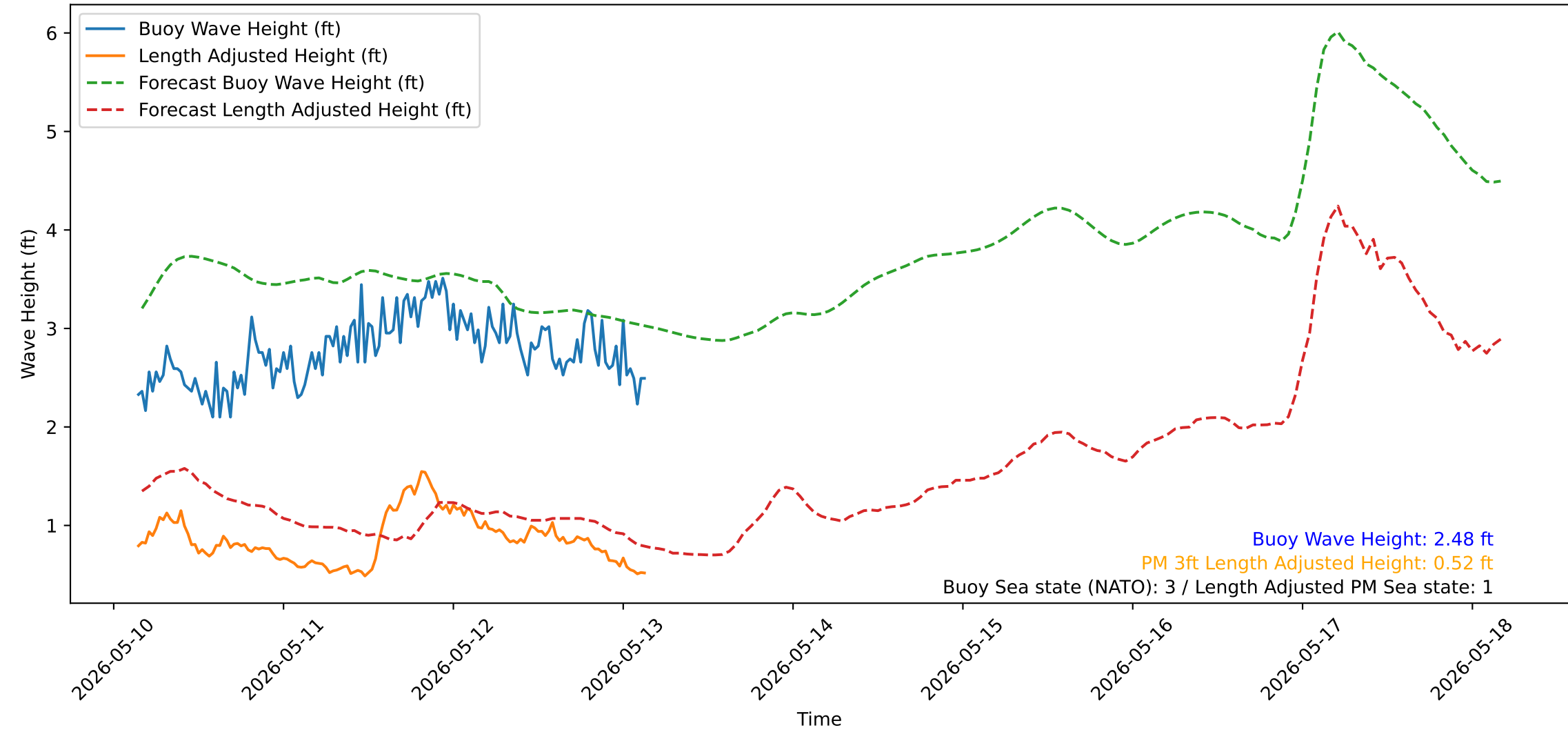
Wave Heights over Time for Green Beach at 2026-05-13 03:41:13
