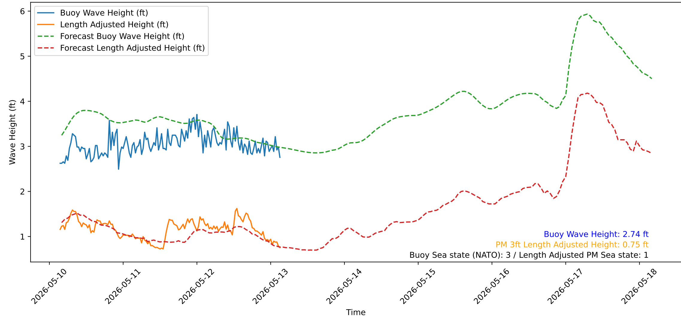
Wave Heights over Time for Oceanside Harbor at 2026-05-13 03:40:31
