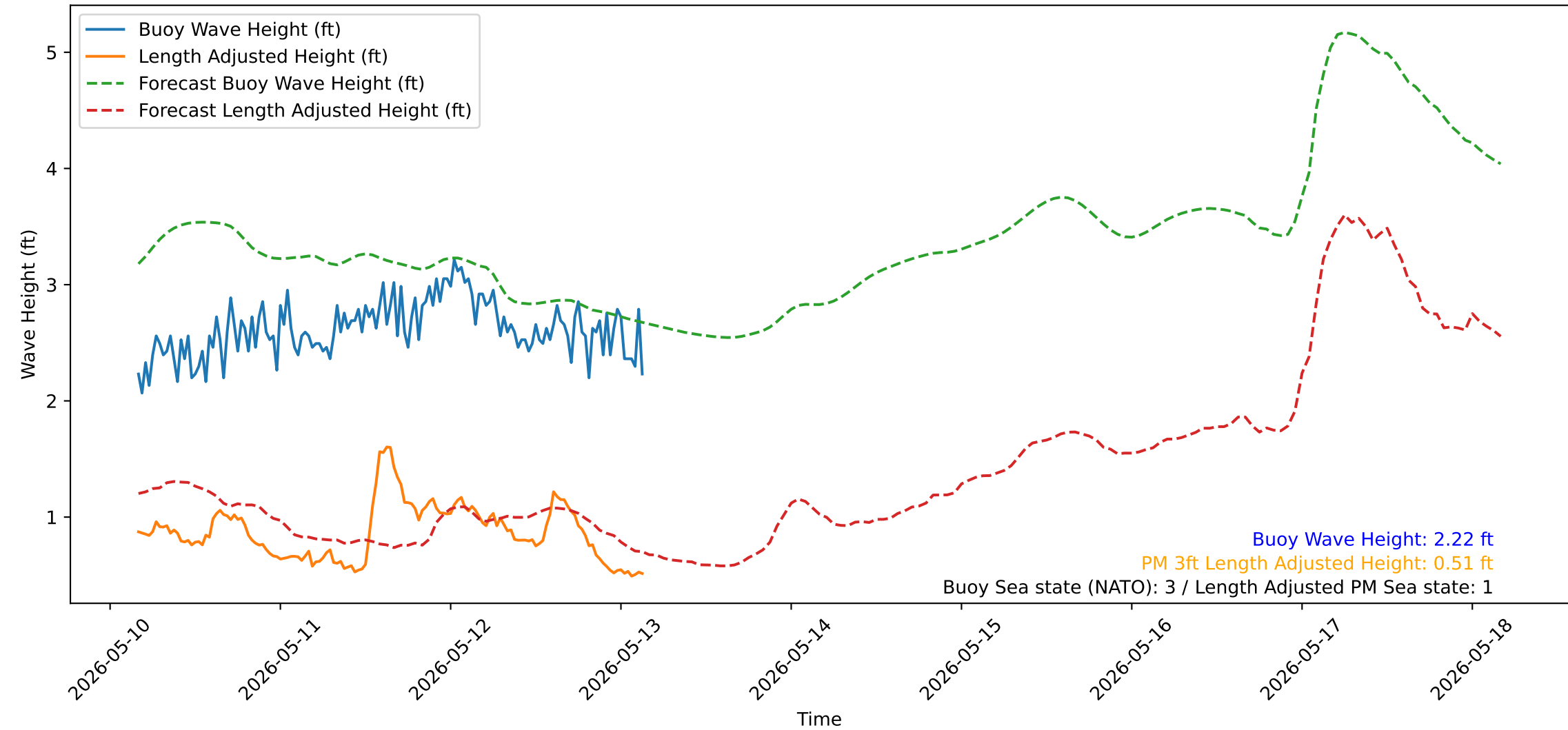
Wave Heights over Time for Red Beach at 2026-05-13 03:40:50
