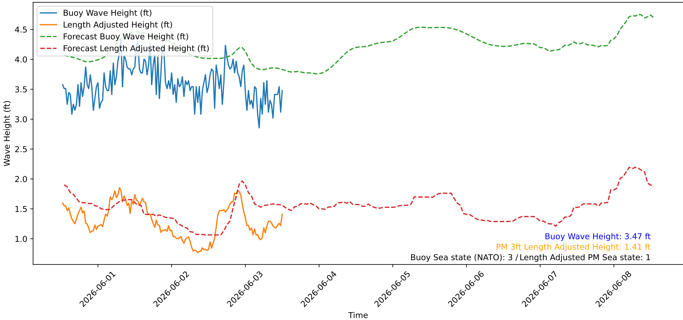
Wave Heights over Time for Green Beach at 2026-06-03 12:41:08
