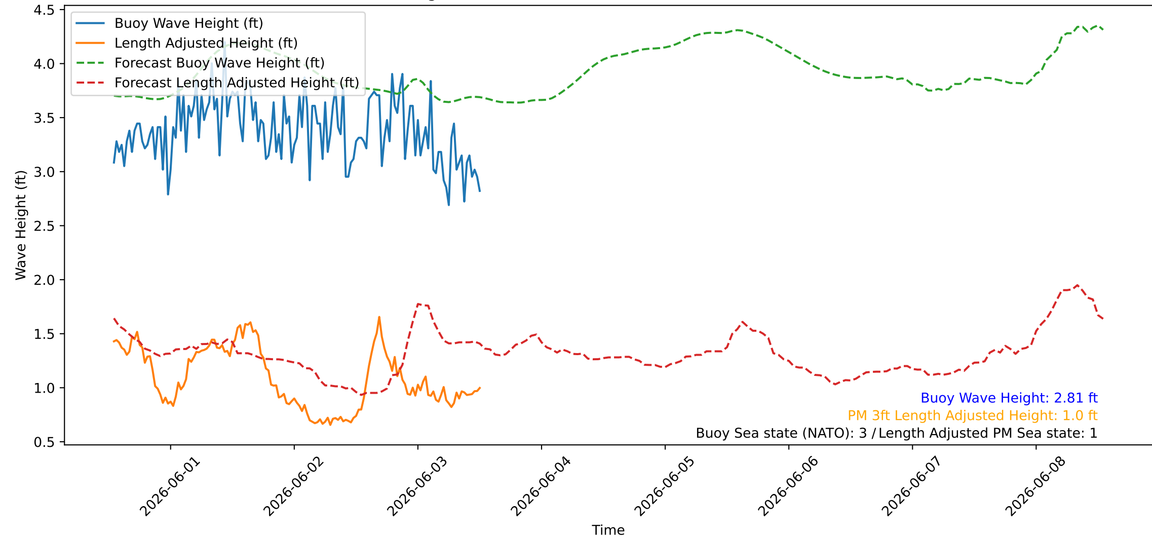
Wave Heights over Time for Red Beach at 2026-06-03 12:40:45
