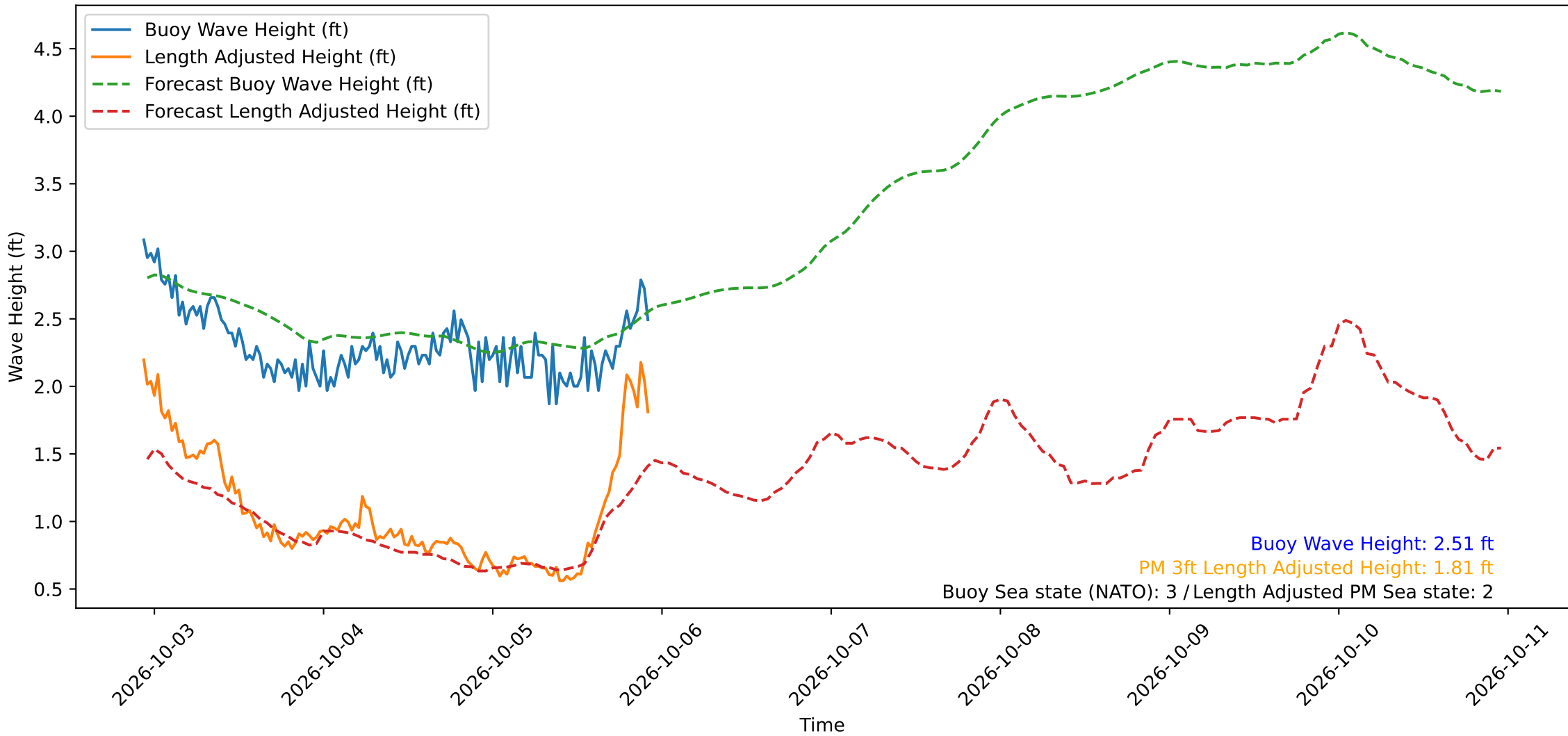
Wave Heights over Time for Oceanside Harbor at 2026-10-05 22:40:29
