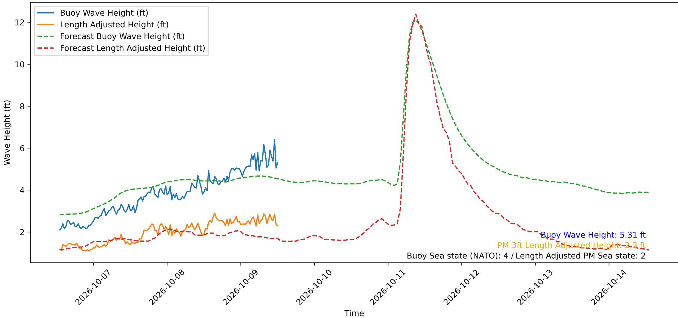
Wave Heights over Time for Oceanside Harbor at 2026-10-09 13:10:29
