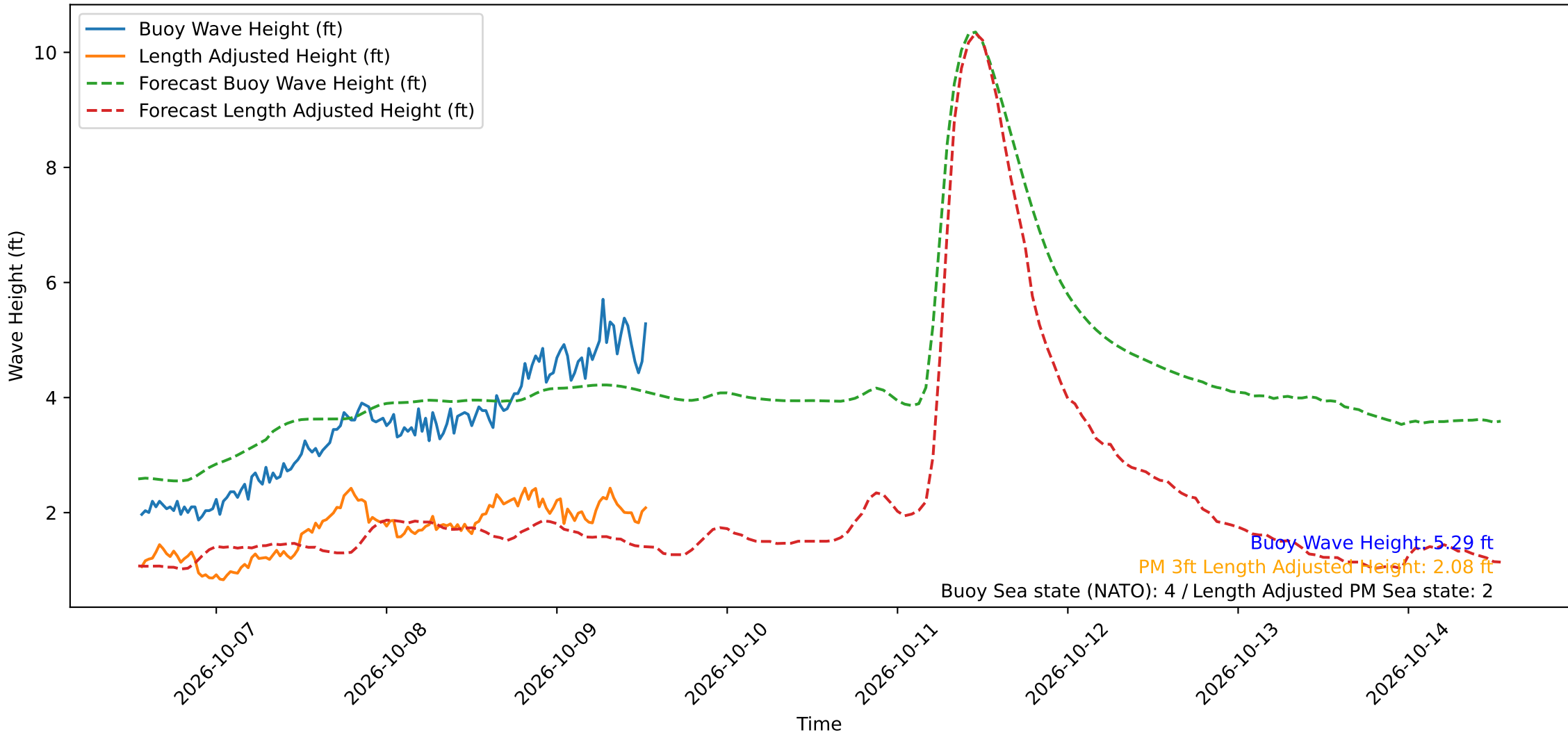
Wave Heights over Time for Red Beach at 2026-10-09 13:10:49
