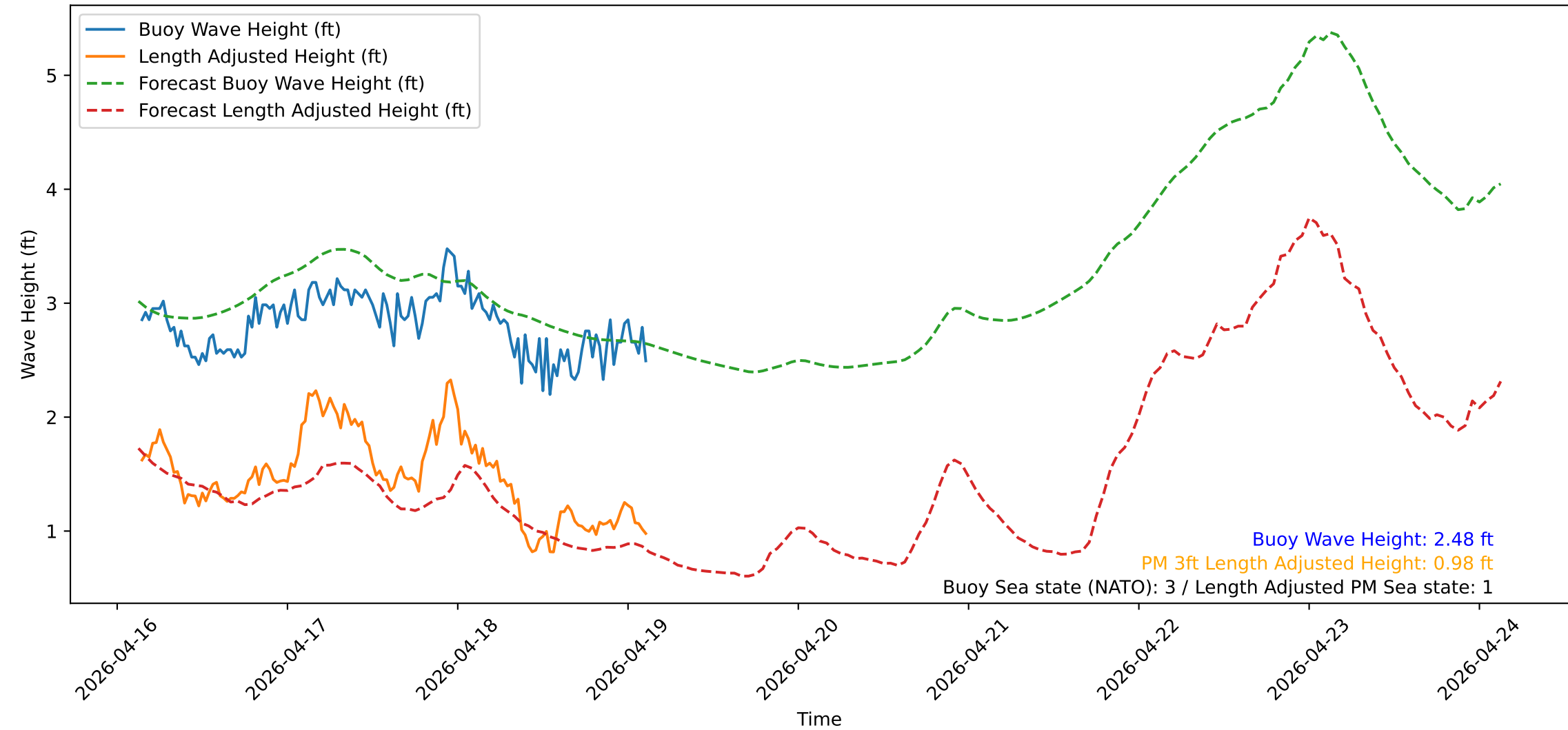
Wave Heights over Time for Green Beach at 2026-04-19 03:21:13
