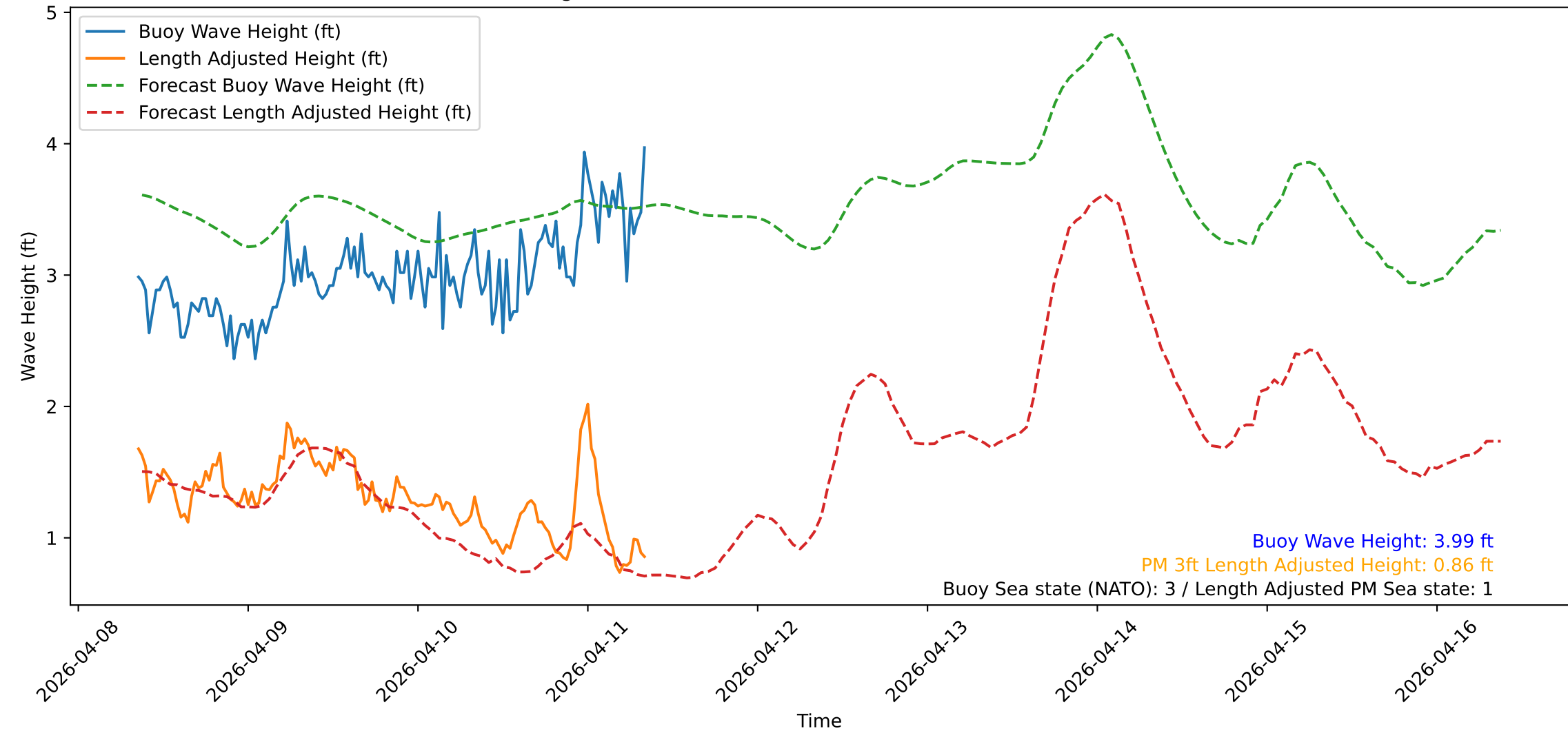
Wave Heights over Time for Green Beach at 2026-04-11 08:41:13
