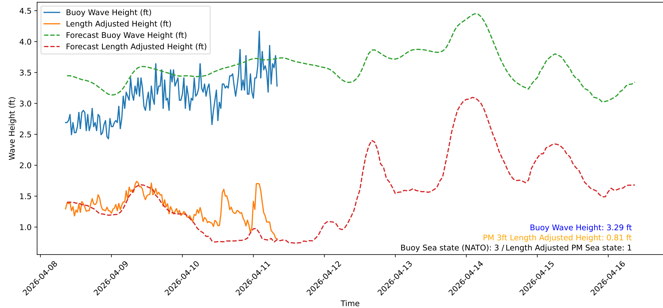
Wave Heights over Time for Oceanside Harbor at 2026-04-11 08:40:31
