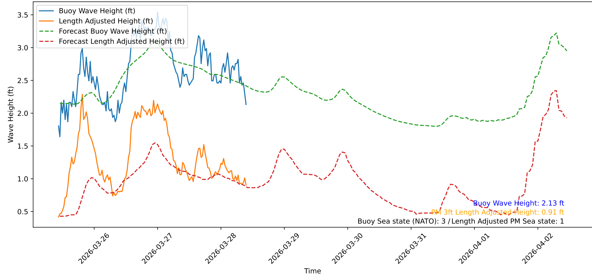
Wave Heights over Time for Green Beach at 2026-03-28 10:31:09
