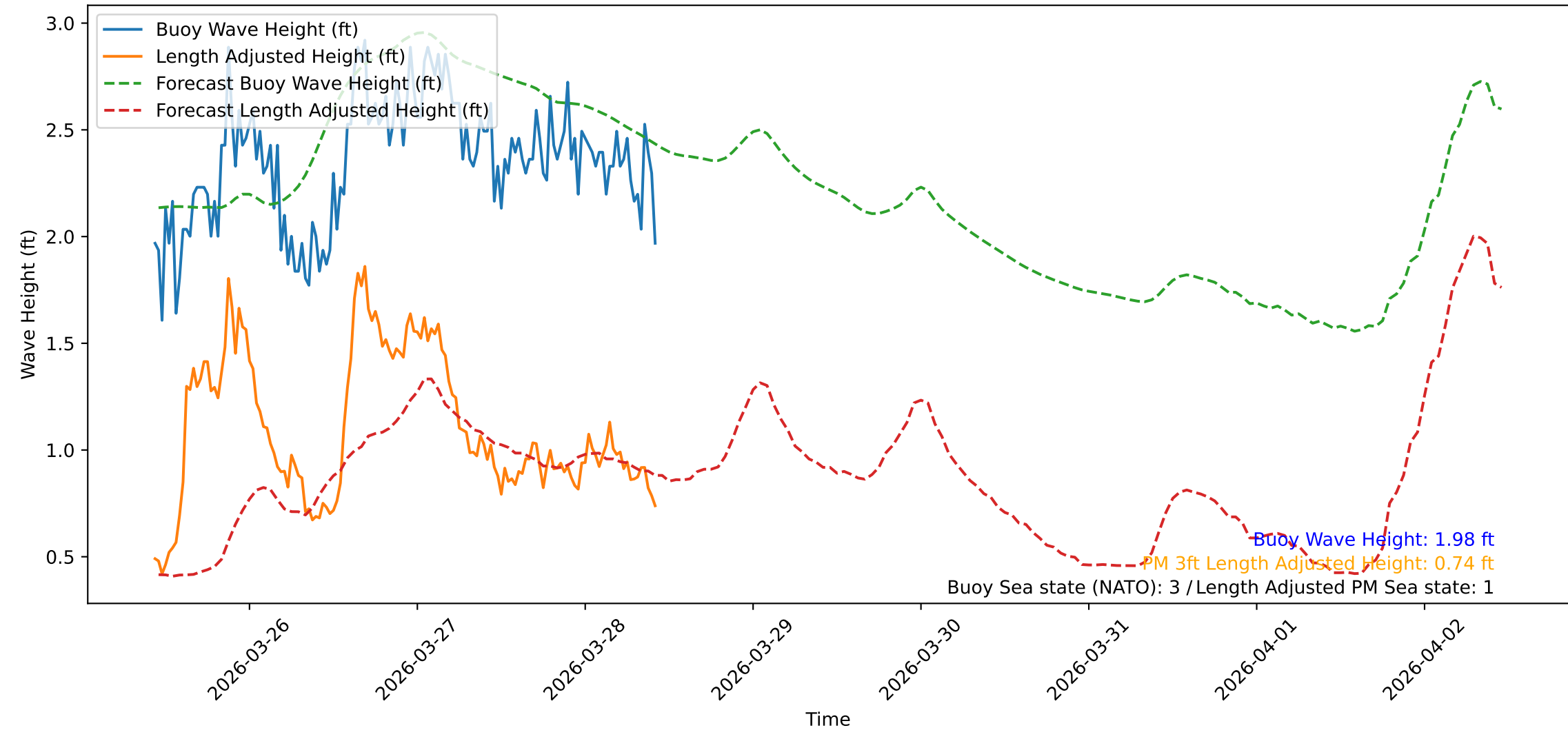
Wave Heights over Time for Oceanside Harbor at 2026-03-28 10:30:31
