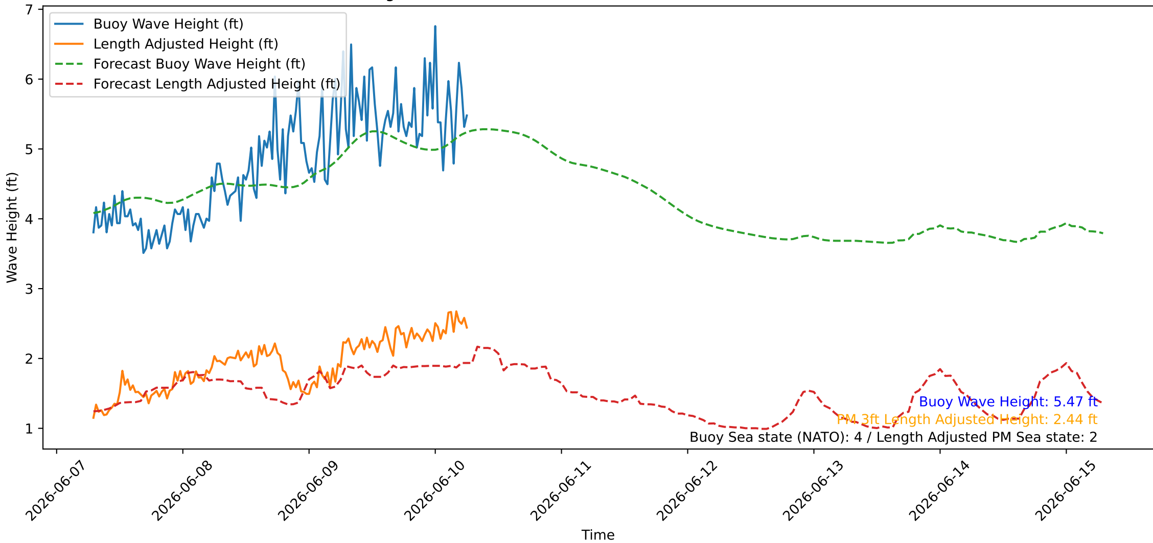
Wave Heights over Time for Oceanside Harbor at 2026-06-10 07:00:26
