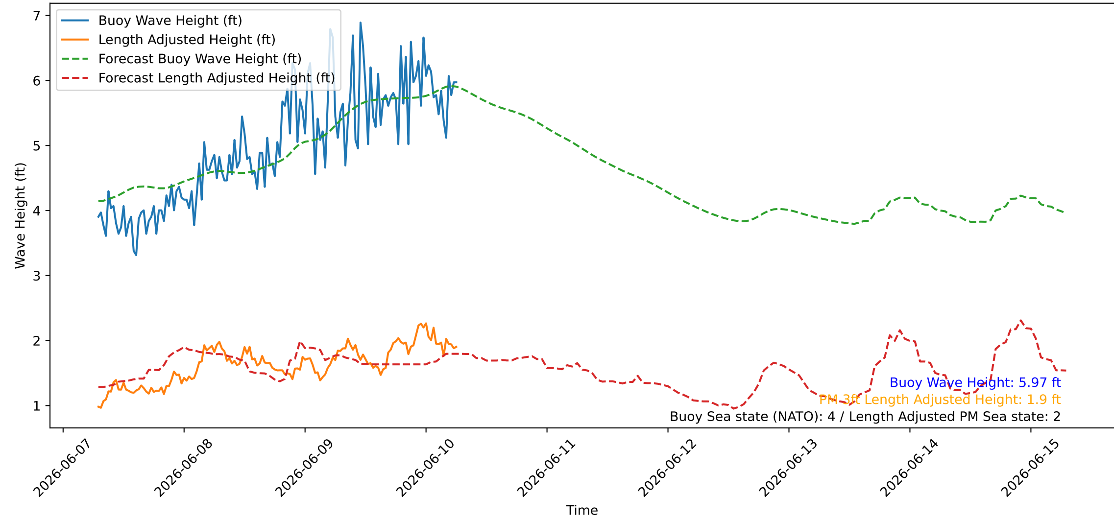
Wave Heights over Time for Green Beach at 2026-06-10 07:01:09
