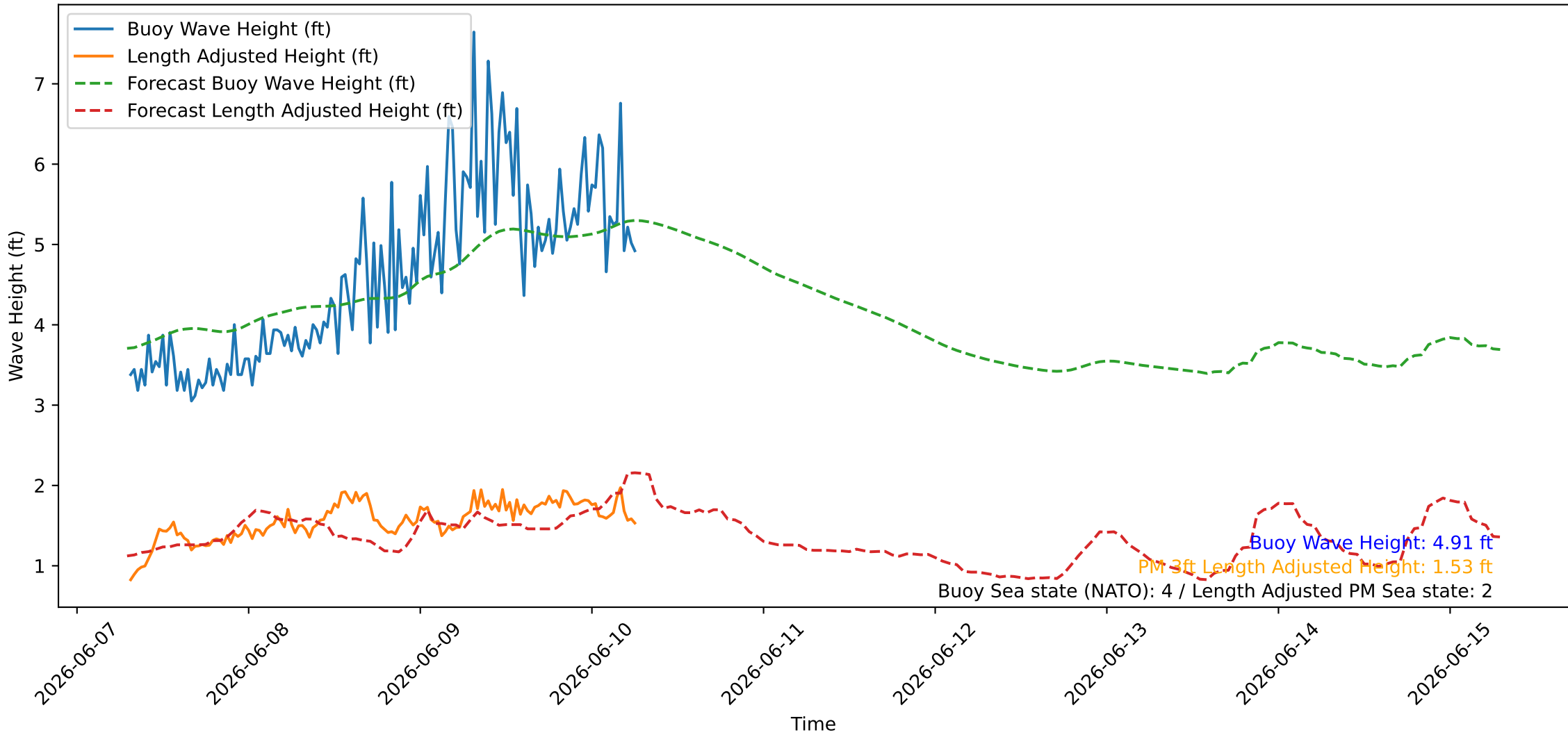
Wave Heights over Time for Red Beach at 2026-06-10 07:00:46
