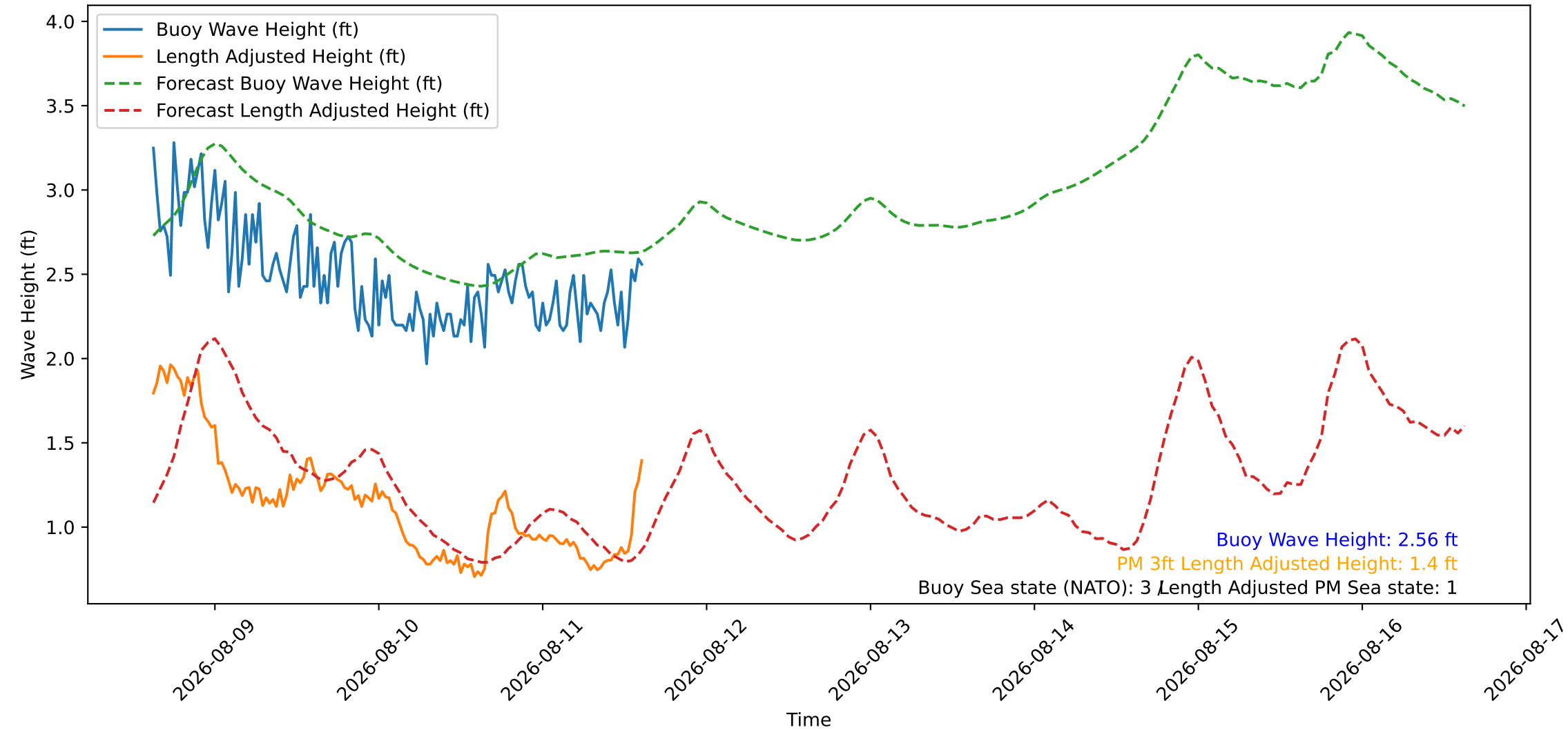
Wave Heights over Time for Oceanside Harbor at 2026-08-11 15:10:27
