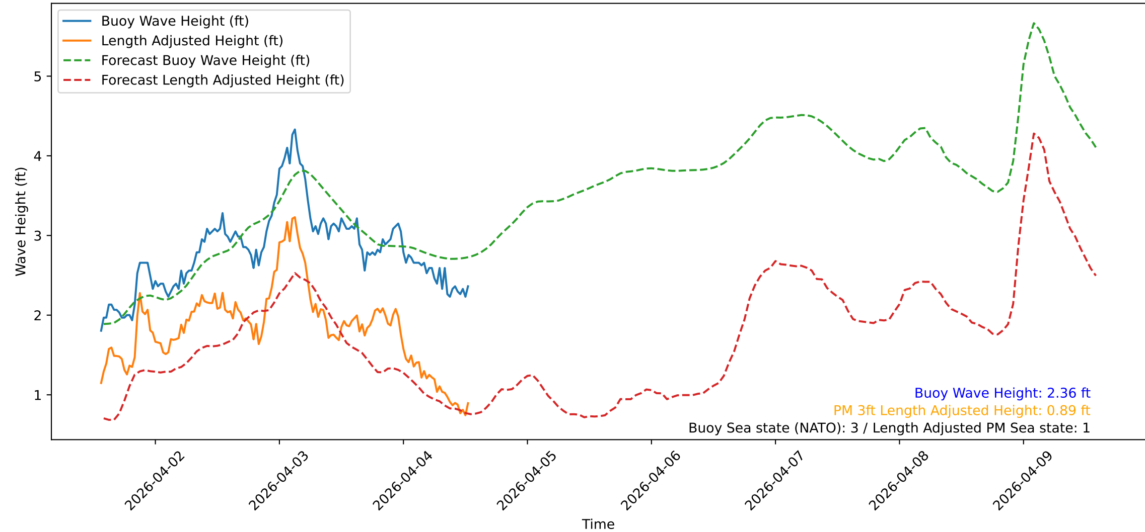
Wave Heights over Time for Green Beach at 2026-04-04 13:31:10
