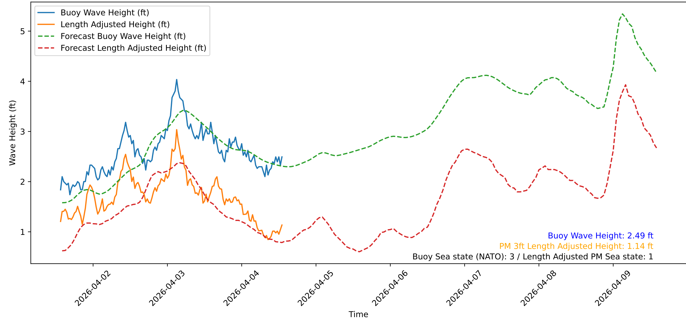
Wave Heights over Time for Oceanside Harbor at 2026-04-04 13:30:32
