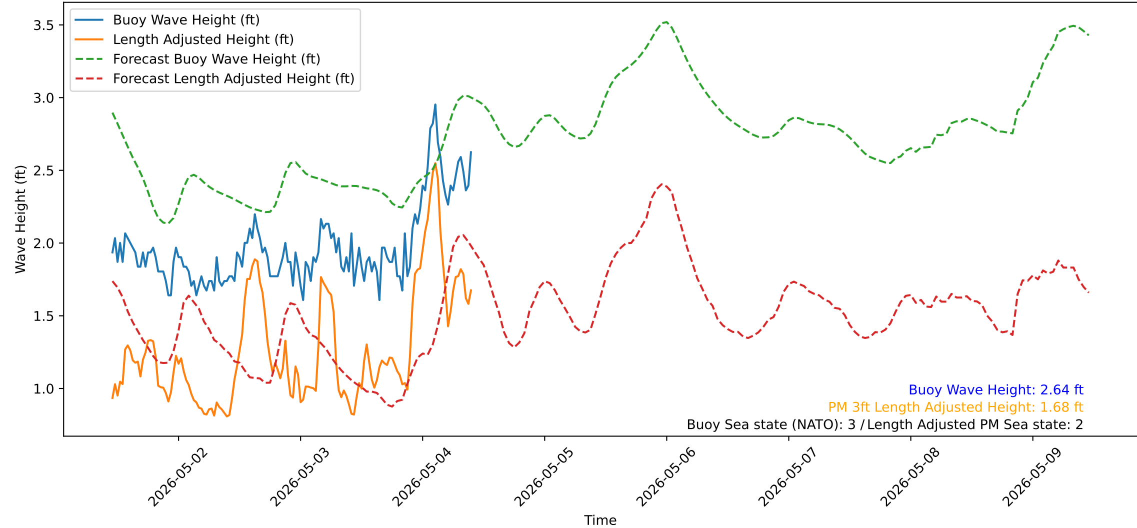
Wave Heights over Time for Red Beach at 2026-05-04 10:30:50
