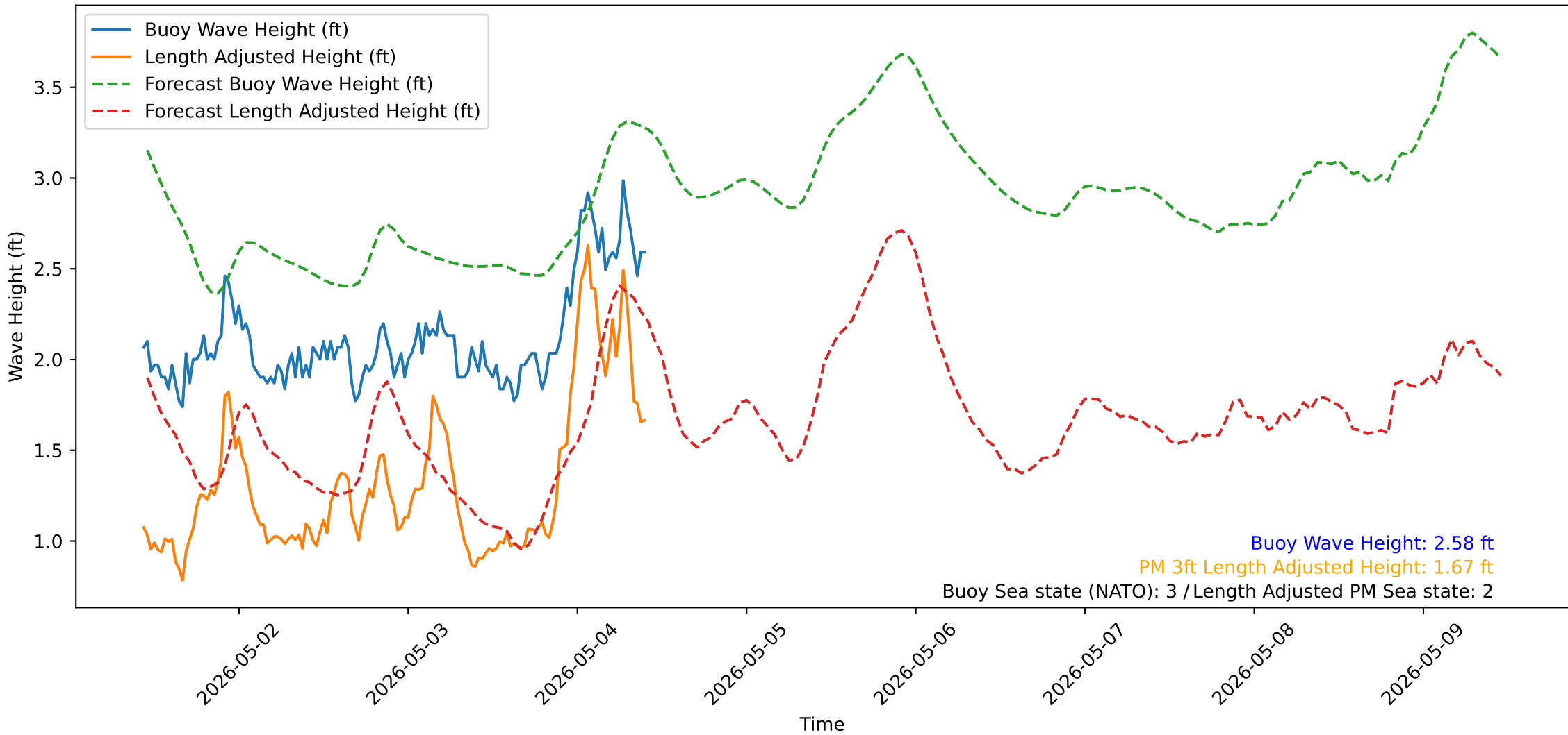
Wave Heights over Time for Green Beach at 2026-05-04 10:31:12
