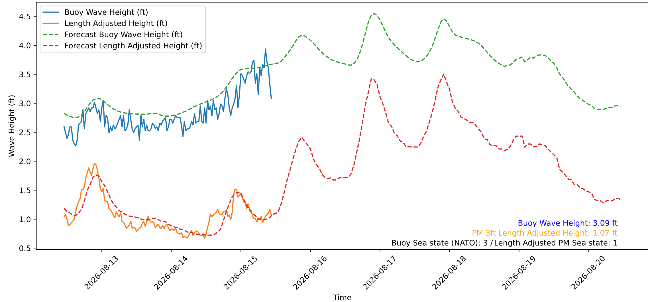
Wave Heights over Time for Green Beach at 2026-08-15 11:11:07
