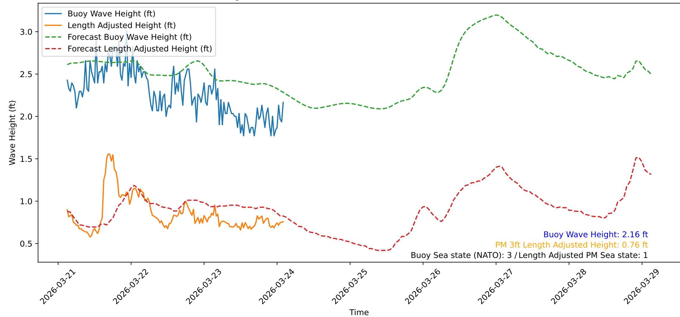
Wave Heights over Time for Oceanside Harbor at 2026-03-24 03:00:31
