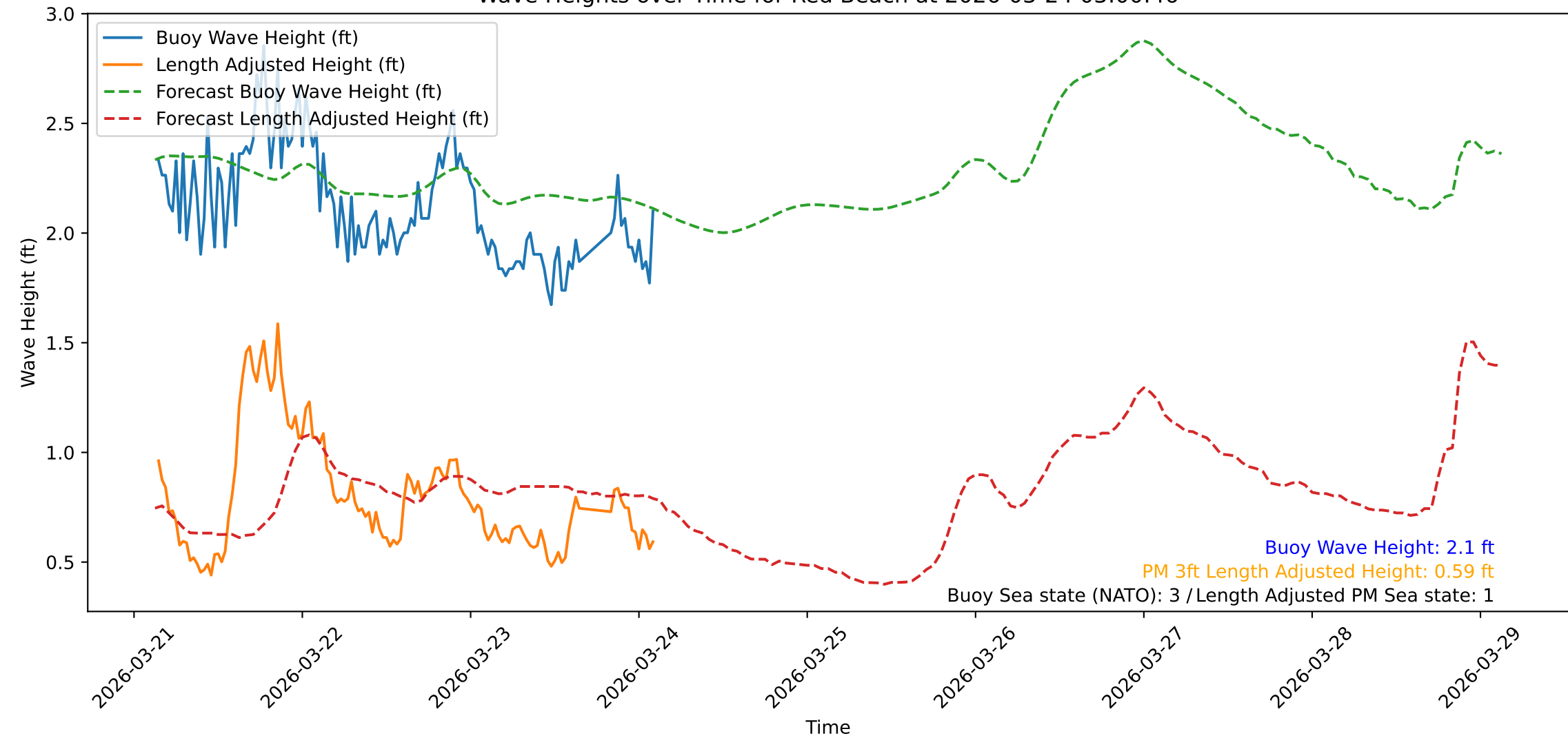
Wave Heights over Time for Red Beach at 2026-03-24 03:00:46
