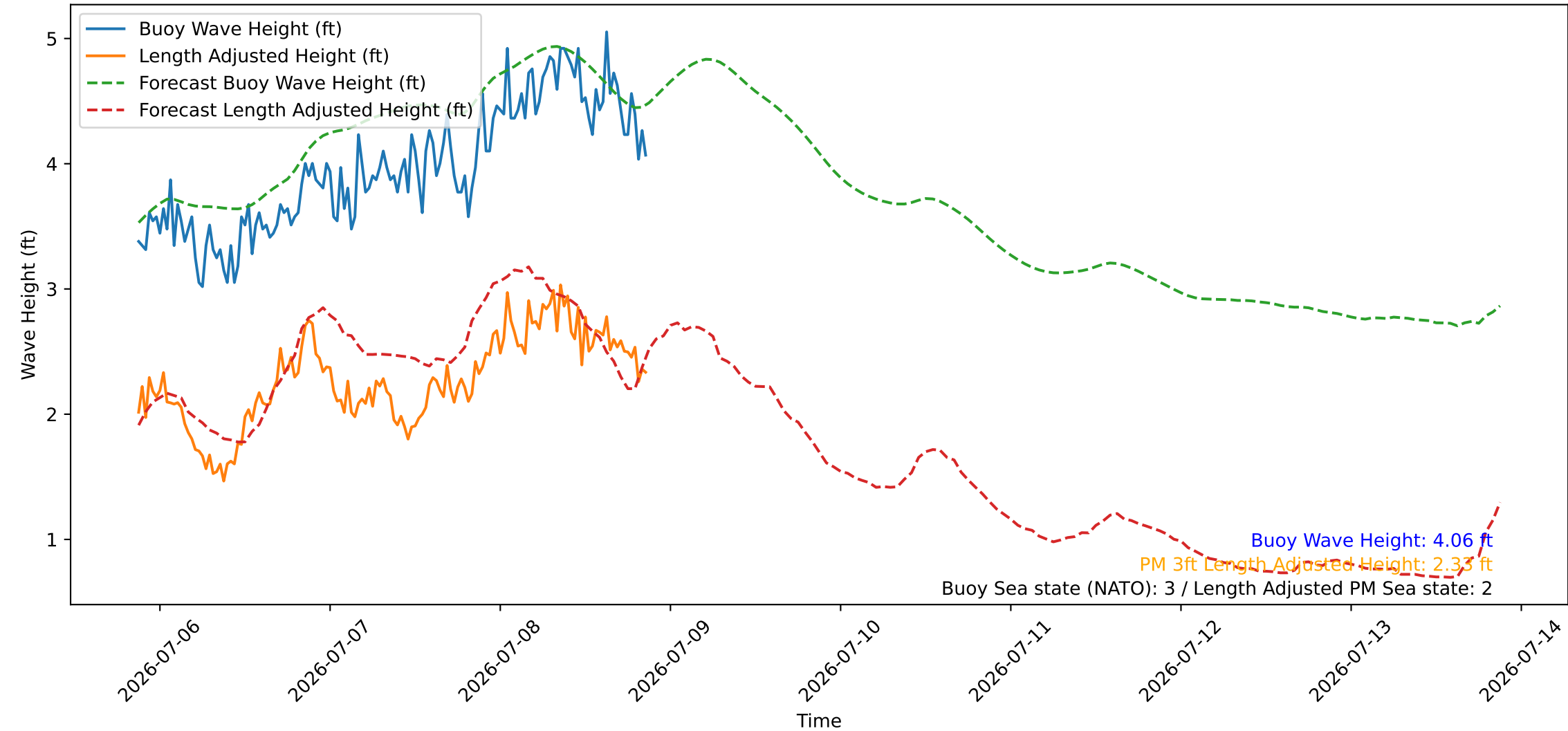
Wave Heights over Time for Oceanside Harbor at 2026-07-08 21:10:26
