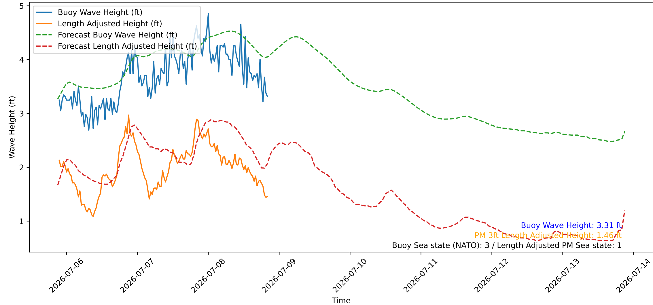
Wave Heights over Time for Red Beach at 2026-07-08 21:10:46
