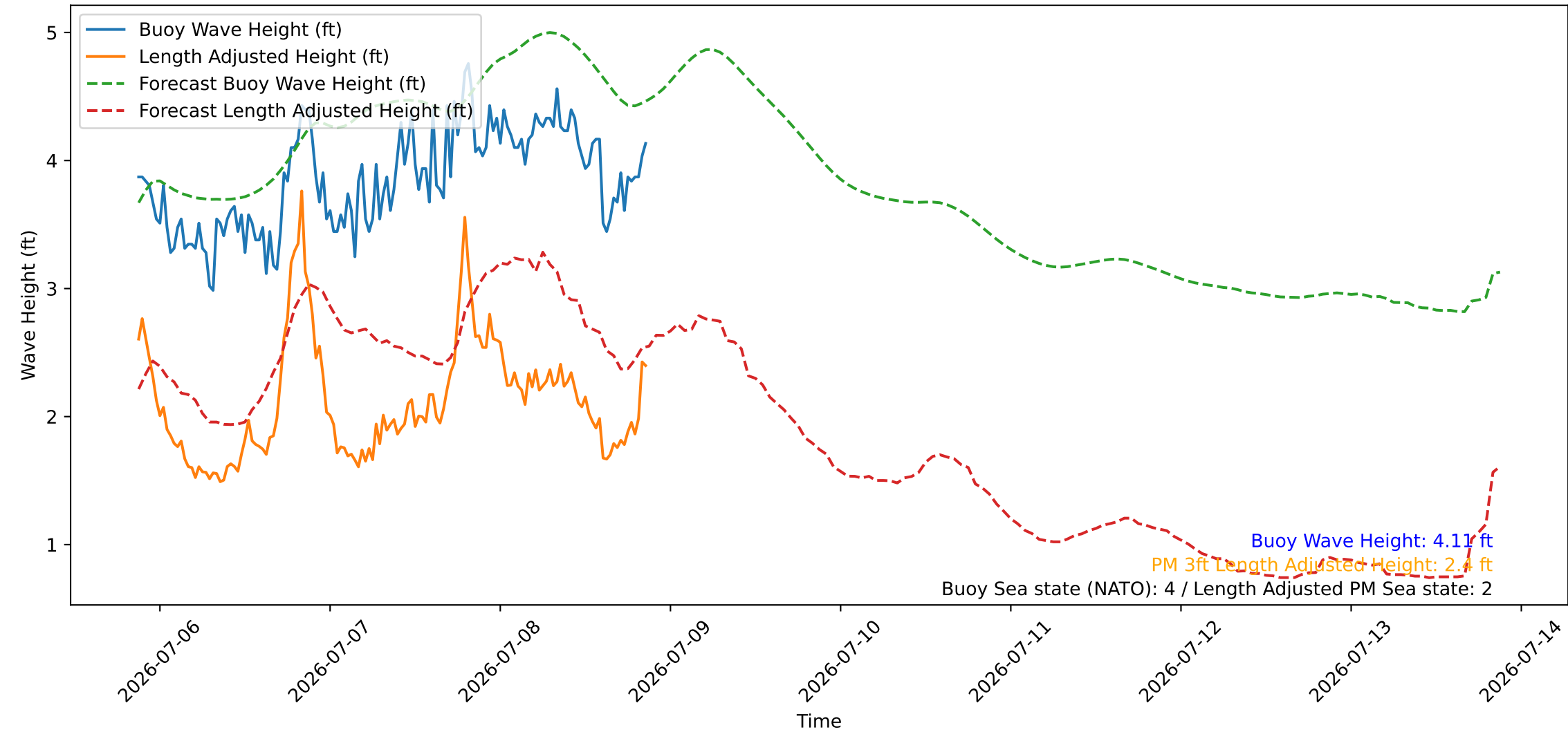
Wave Heights over Time for Green Beach at 2026-07-08 21:11:08
