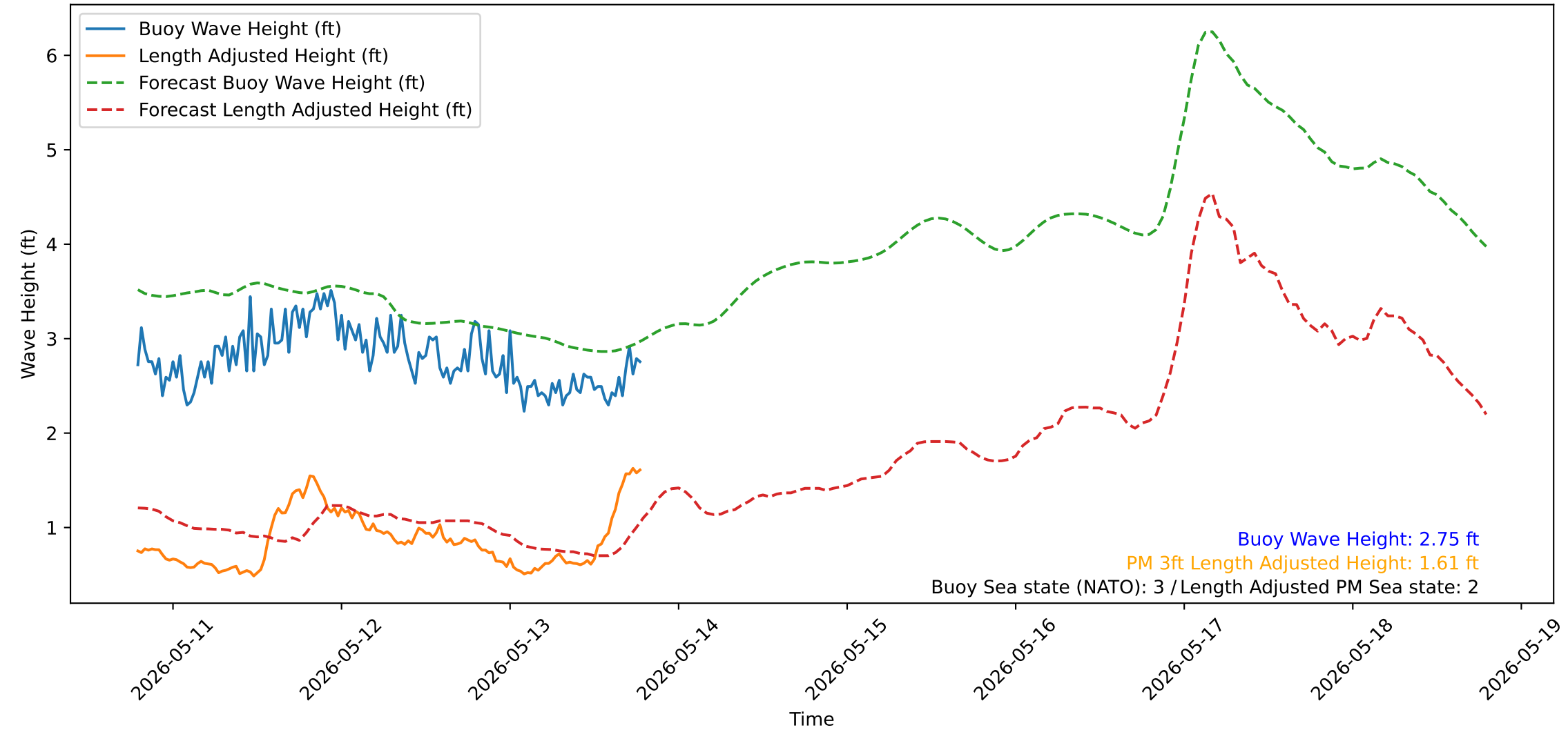
Wave Heights over Time for Green Beach at 2026-05-13 19:11:14
