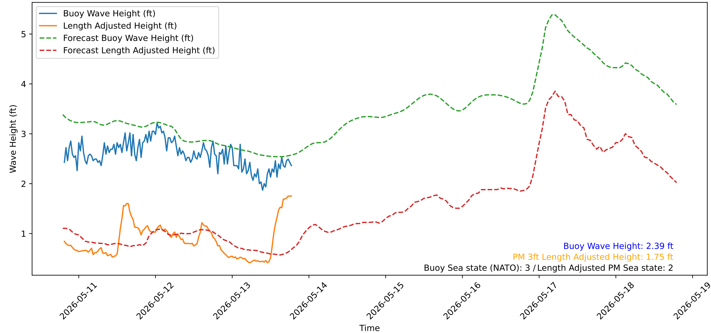
Wave Heights over Time for Red Beach at 2026-05-13 19:10:51
