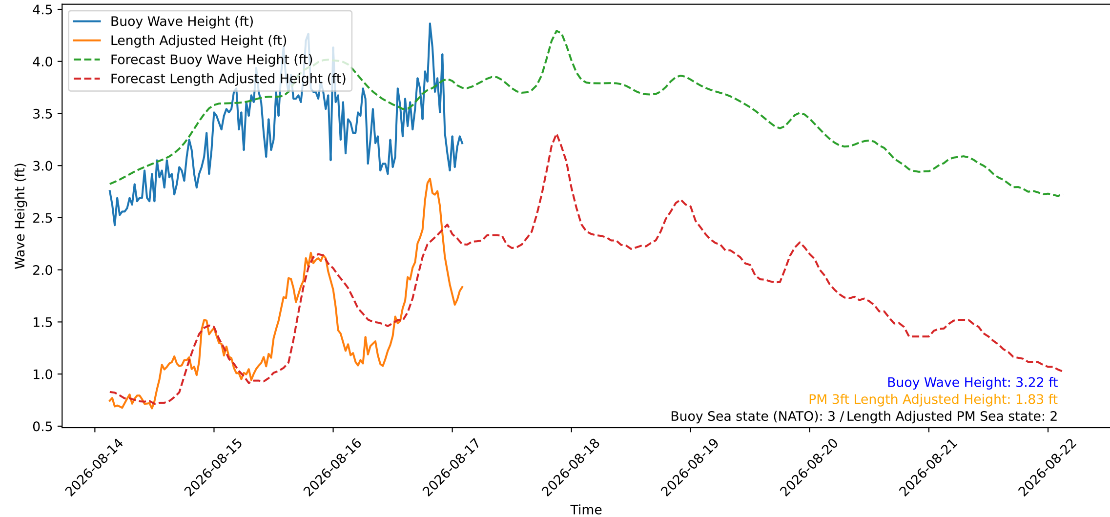
Wave Heights over Time for Green Beach at 2026-08-17 02:41:17
