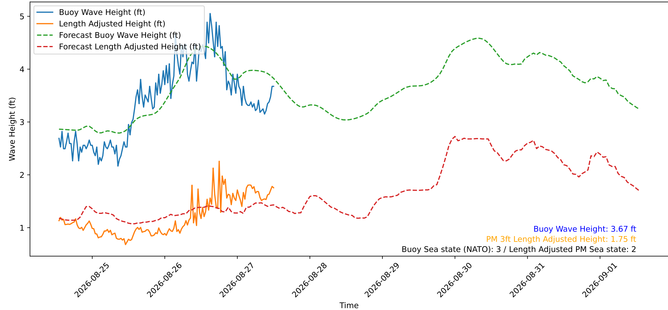
Wave Heights over Time for Red Beach at 2026-08-27 12:50:52
