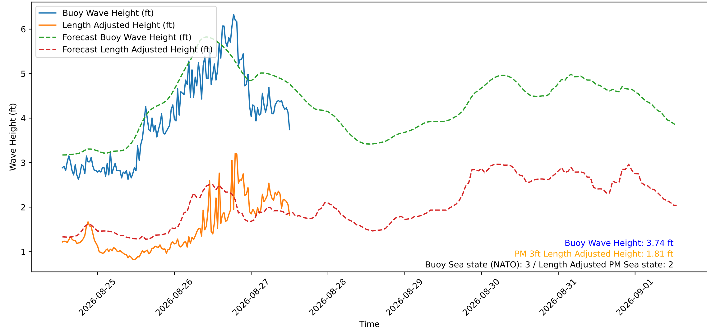
Wave Heights over Time for Green Beach at 2026-08-27 12:51:17
