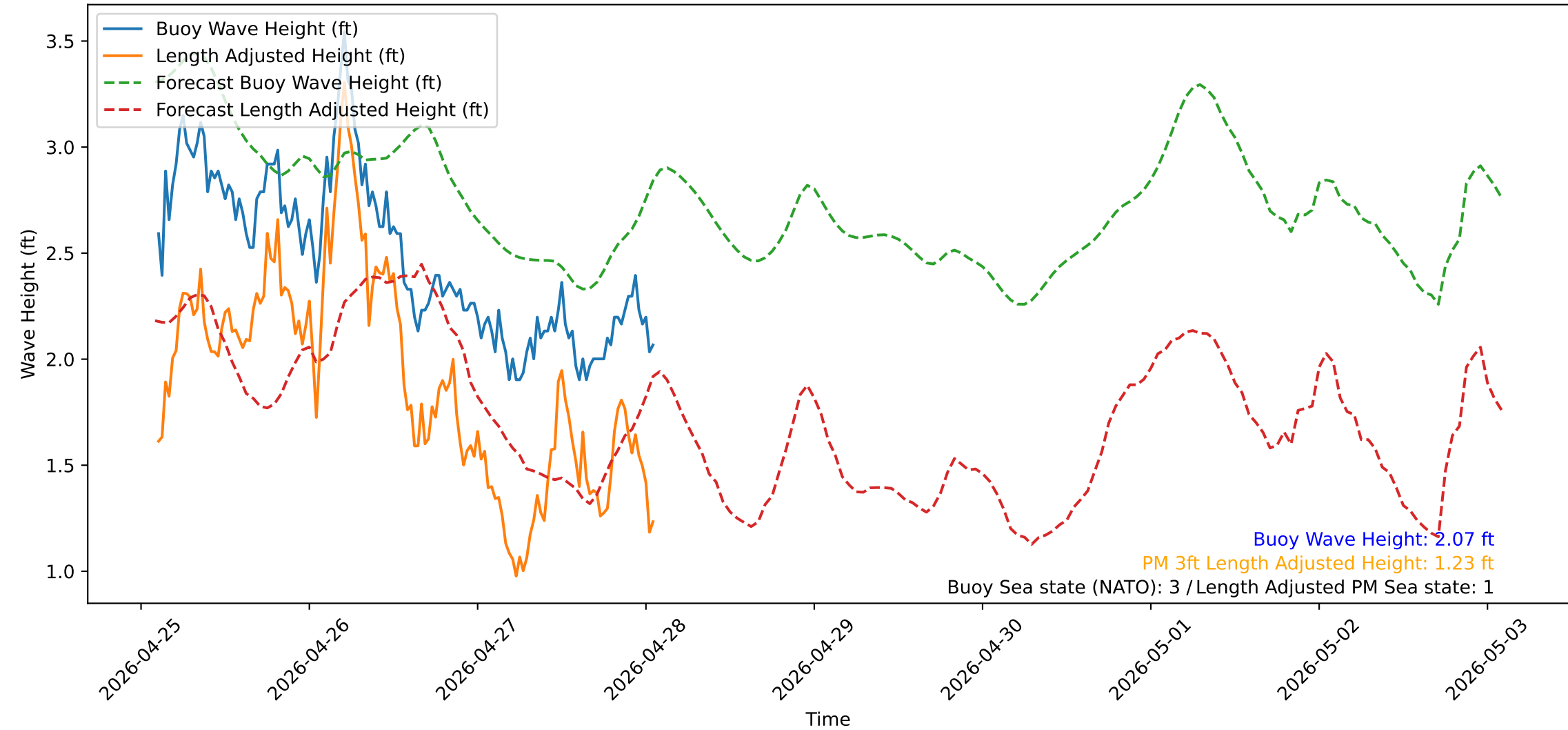
Wave Heights over Time for Red Beach at 2026-04-28 02:00:49
