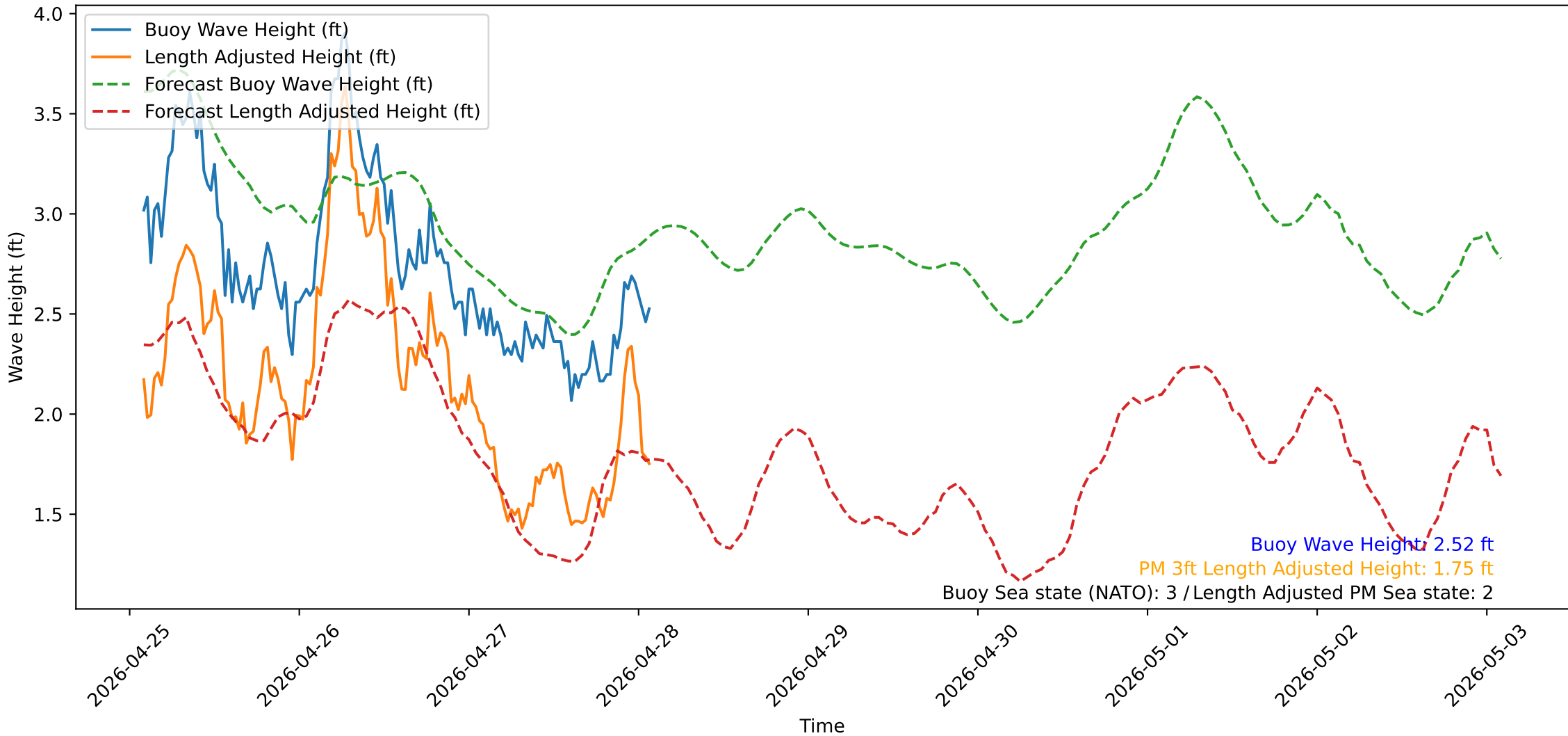
Wave Heights over Time for Oceanside Harbor at 2026-04-28 02:00:30
