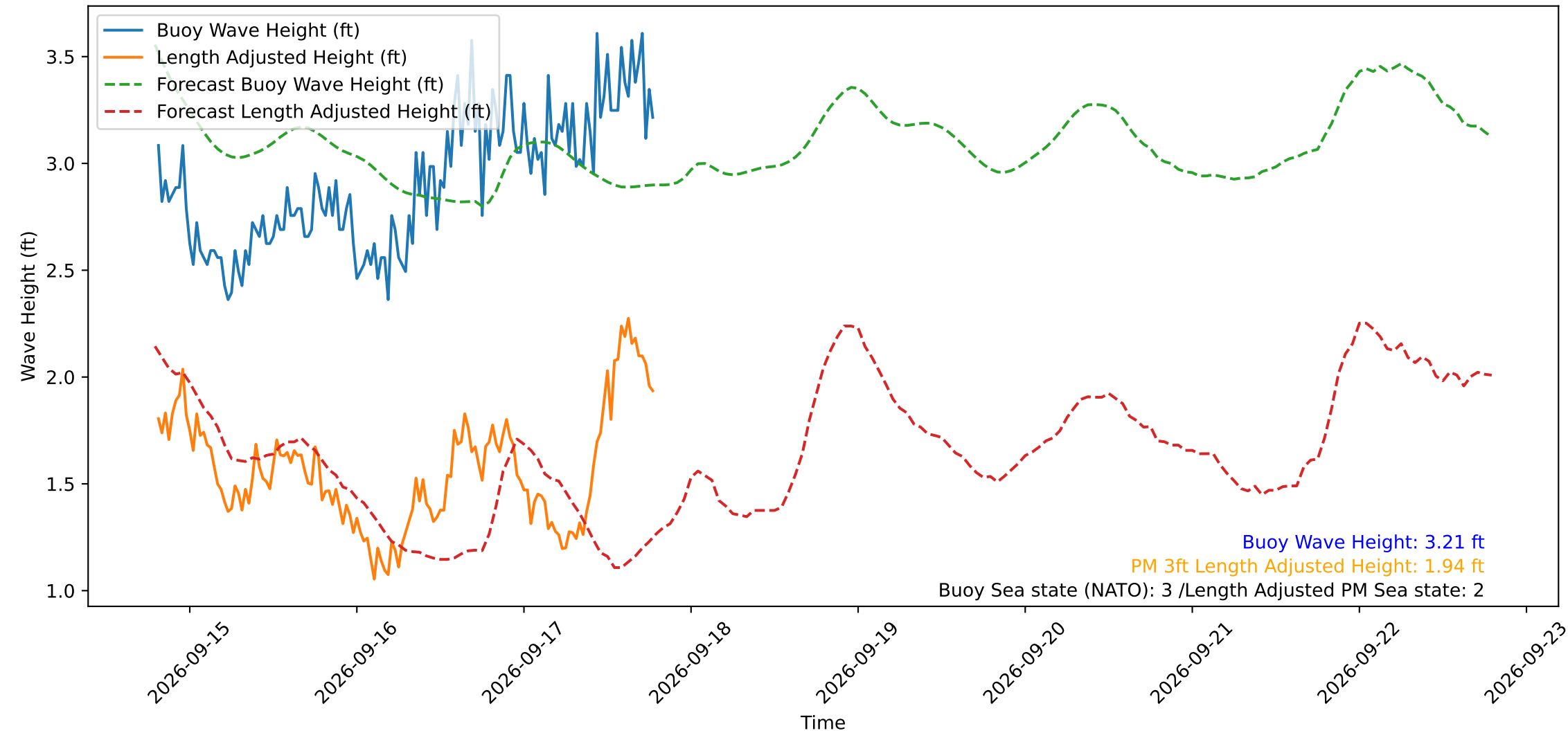
Wave Heights over Time for Oceanside Harbor at 2026-09-17 19:20:29
