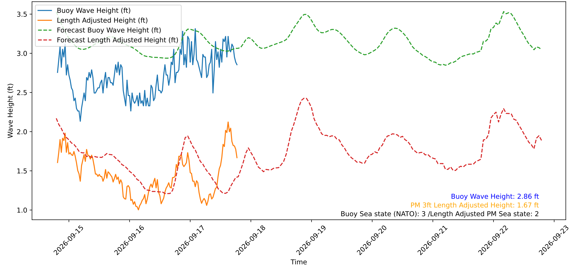
Wave Heights over Time for Green Beach at 2026-09-17 19:21:14
