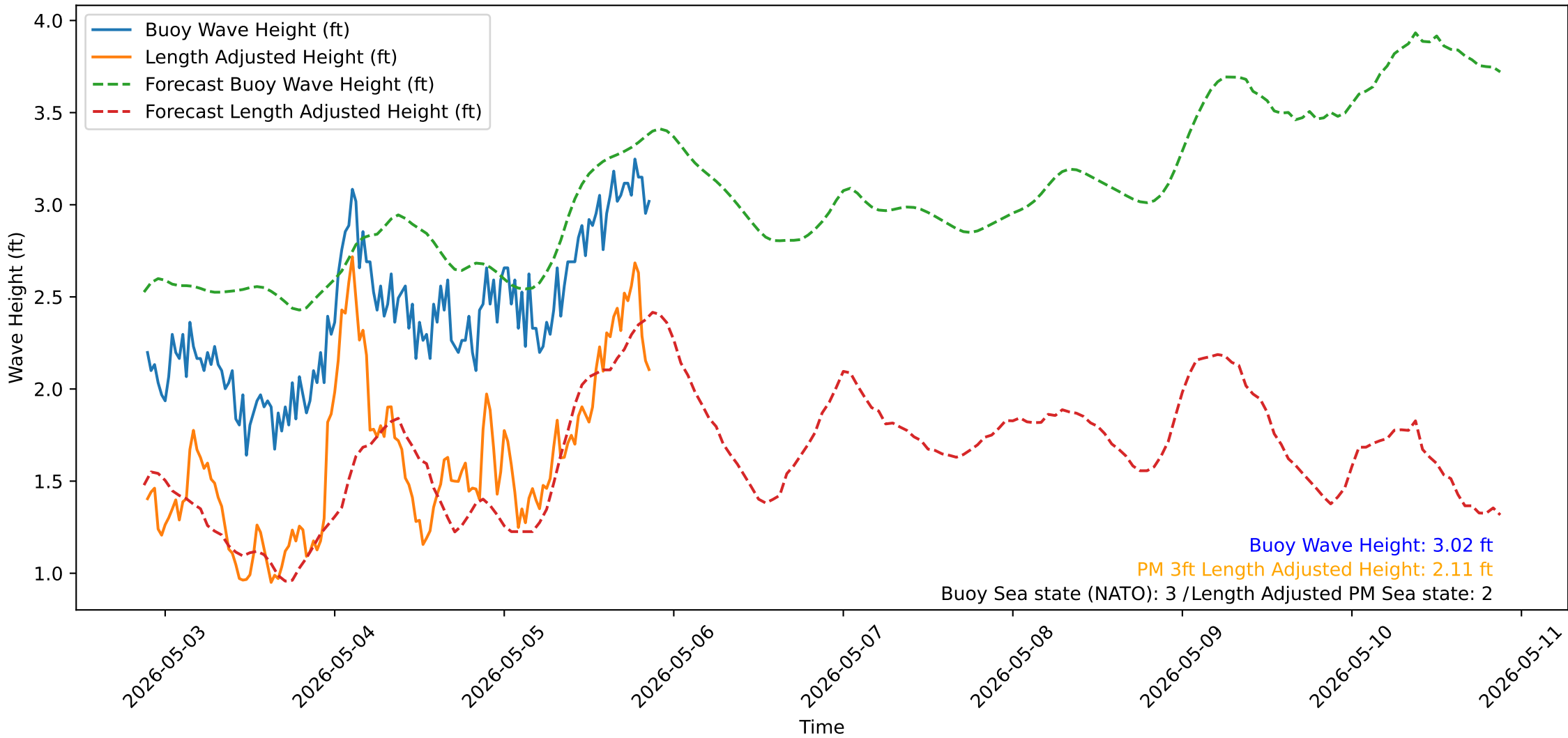
Wave Heights over Time for Oceanside Harbor at 2026-05-05 21:20:31
