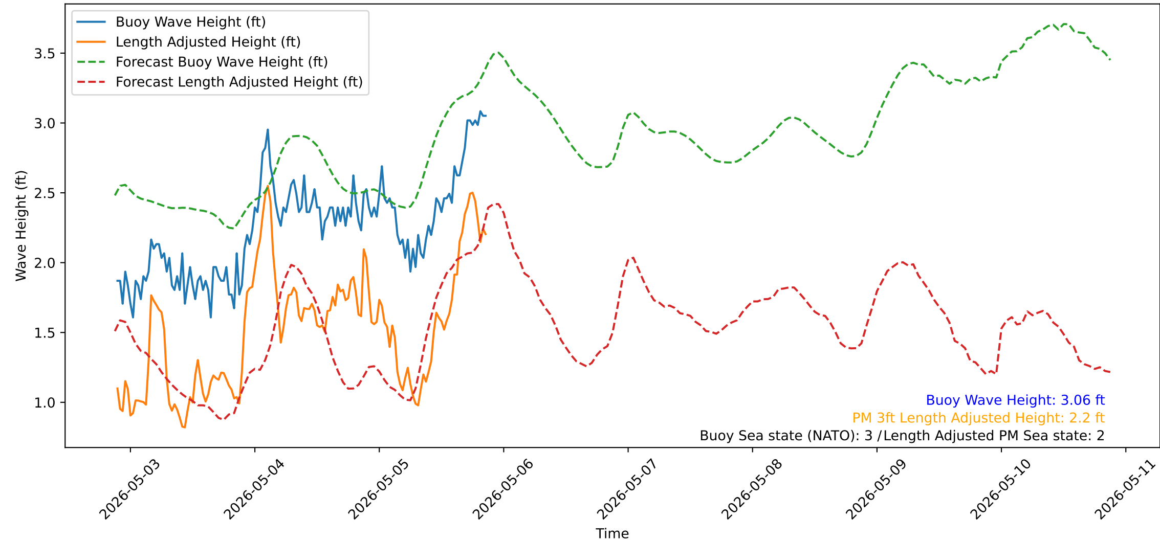
Wave Heights over Time for Red Beach at 2026-05-05 21:20:51
