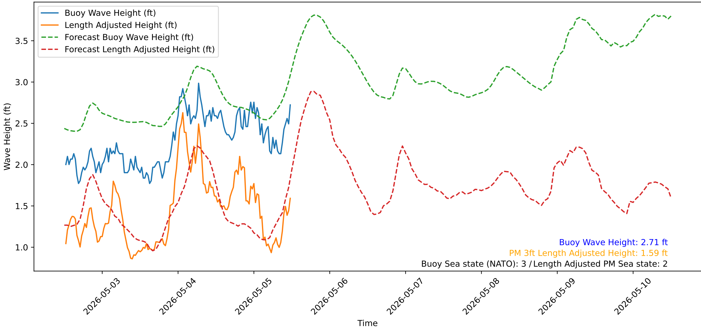
Wave Heights over Time for Green Beach at 2026-05-05 12:21:14
