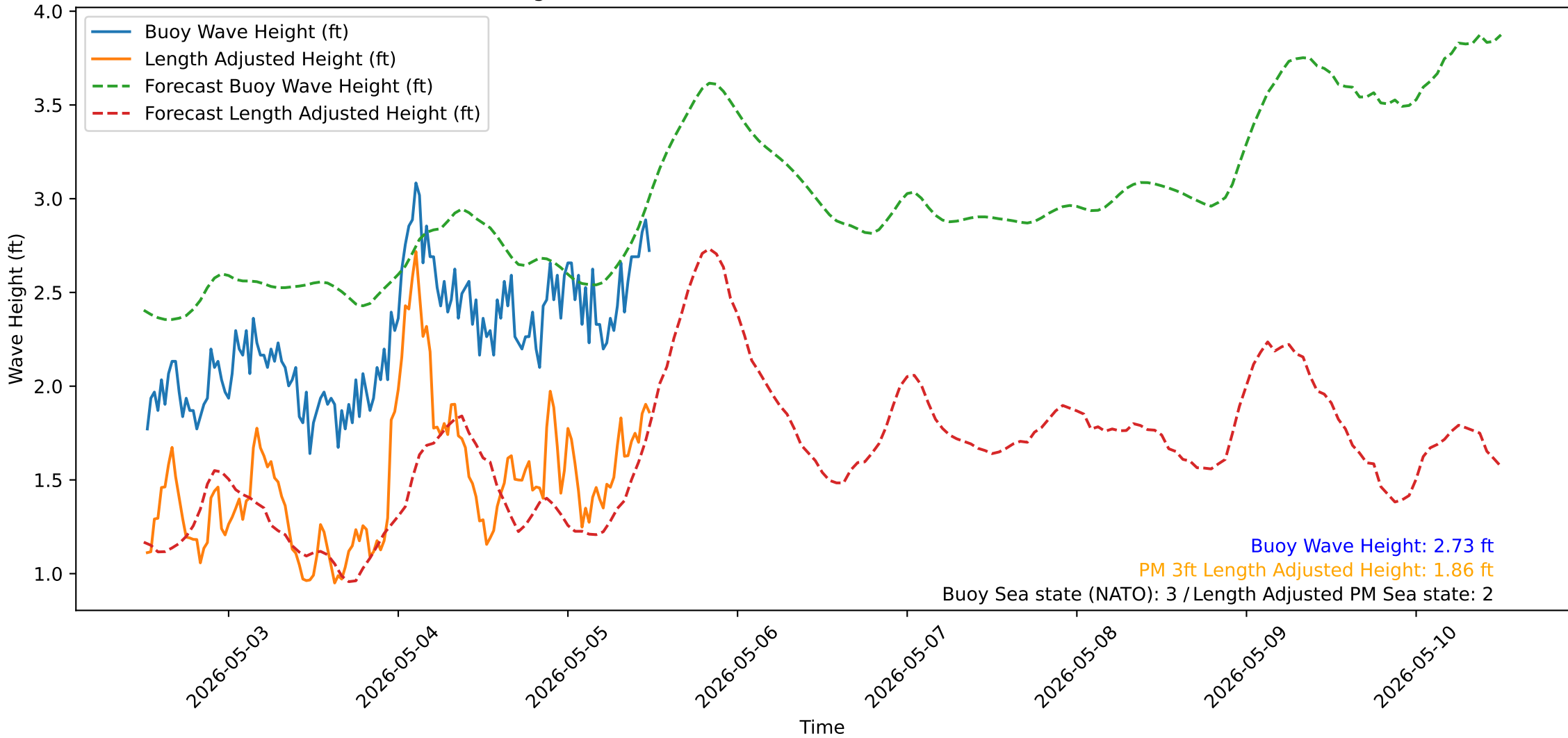
Wave Heights over Time for Oceanside Harbor at 2026-05-05 12:20:31
