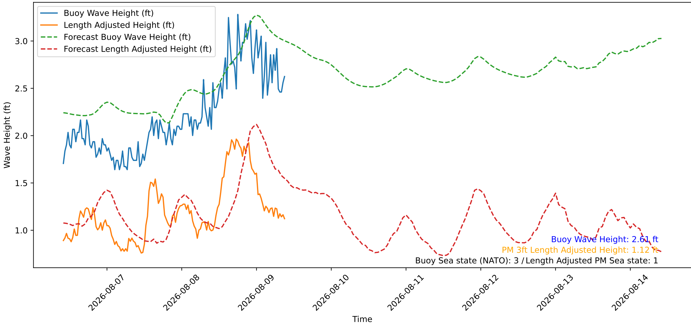
Wave Heights over Time for Oceanside Harbor at 2026-08-09 10:00:26
