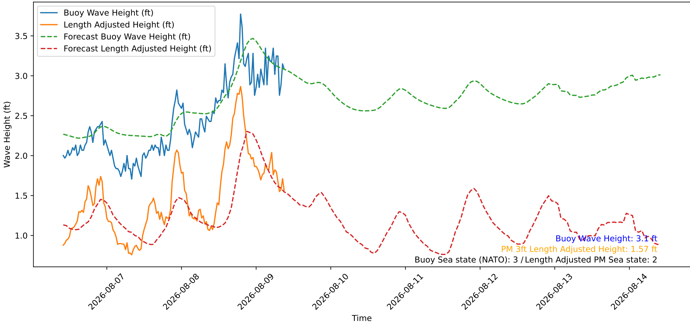
Wave Heights over Time for Green Beach at 2026-08-09 10:01:09
