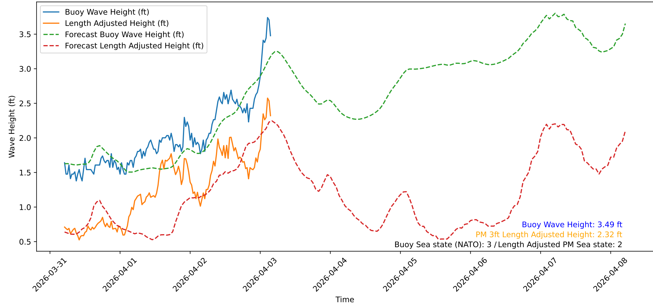
Wave Heights over Time for Red Beach at 2026-04-03 04:30:47
