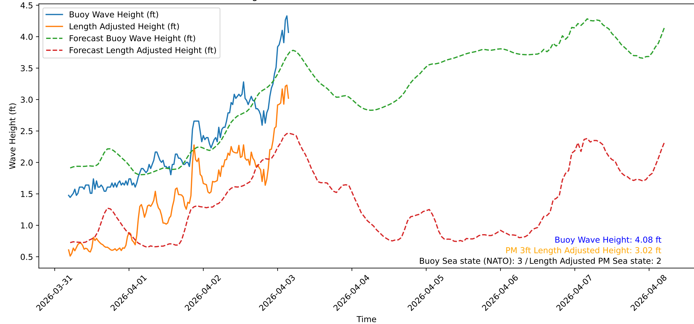
Wave Heights over Time for Green Beach at 2026-04-03 04:31:10
