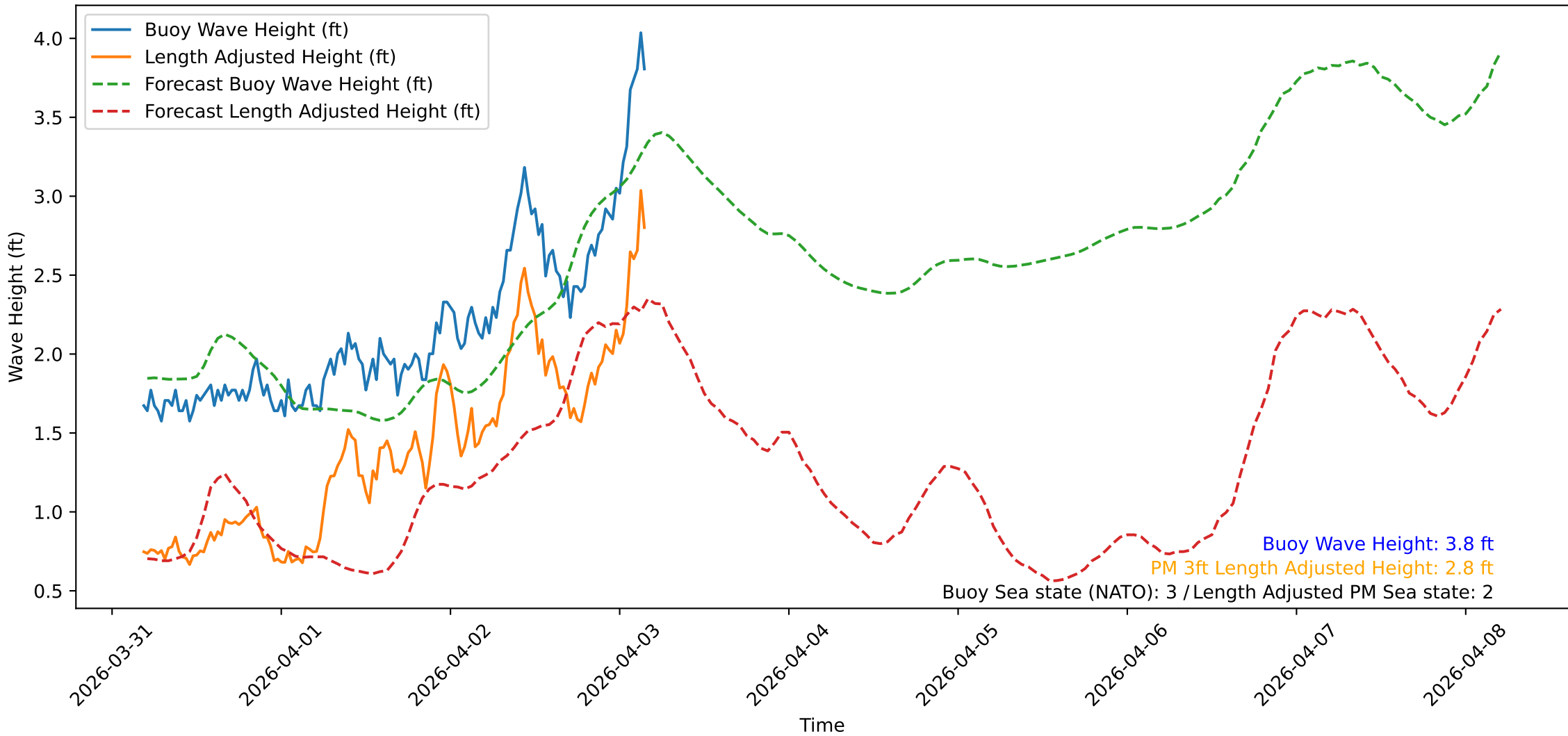
Wave Heights over Time for Oceanside Harbor at 2026-04-03 04:30:31
