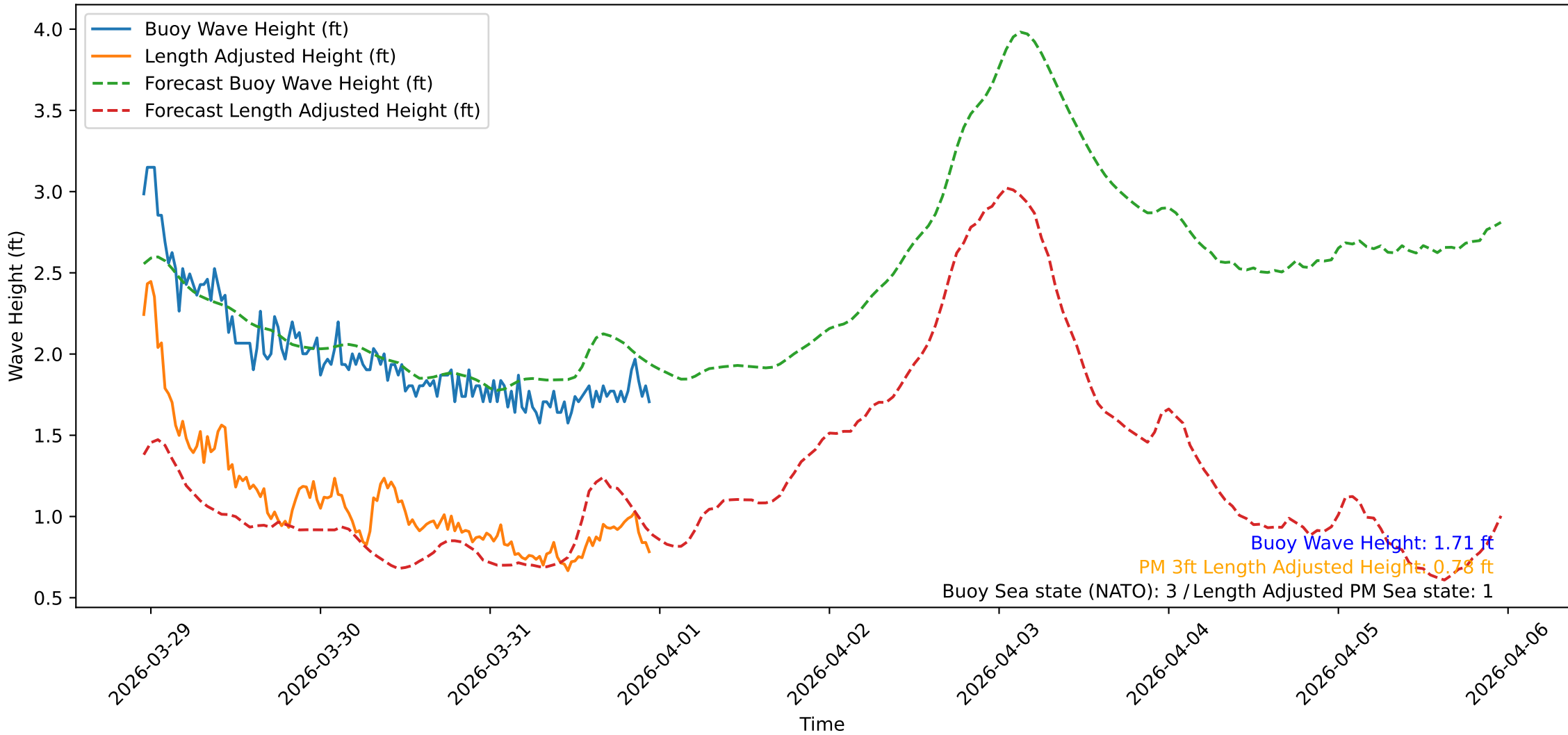
Wave Heights over Time for Oceanside Harbor at 2026-03-31 23:10:31
