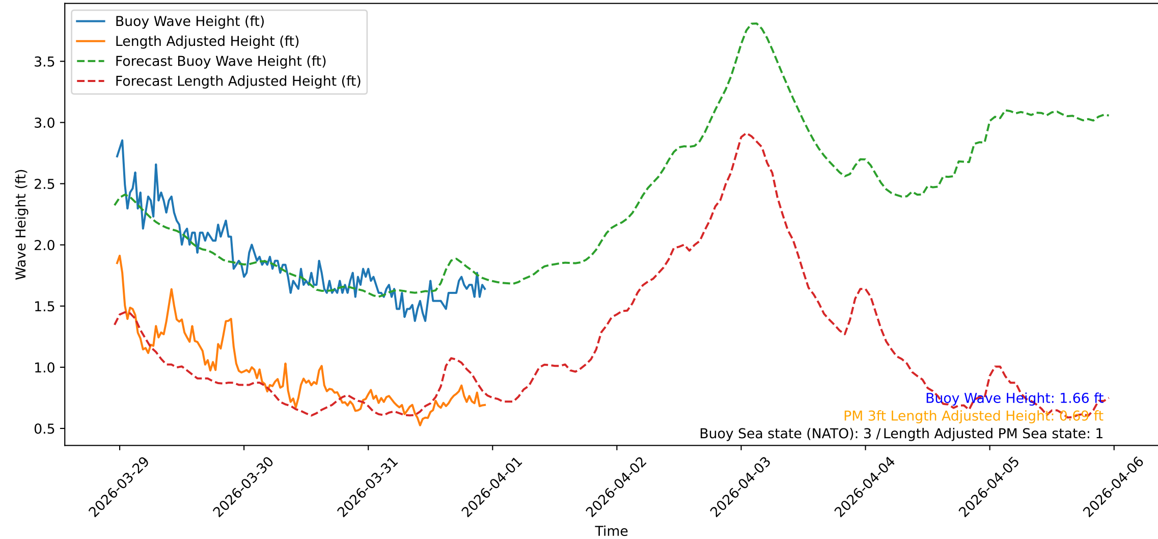
Wave Heights over Time for Red Beach at 2026-03-31 23:10:47
