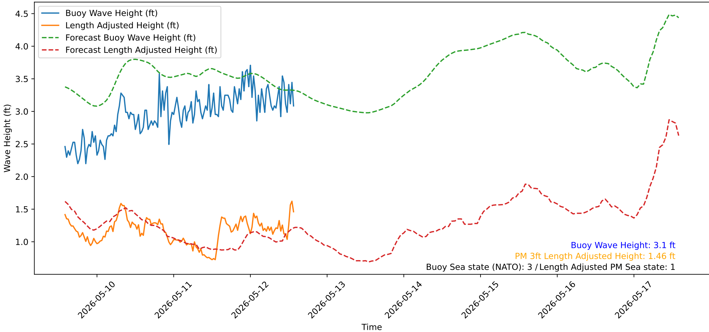
Wave Heights over Time for Oceanside Harbor at 2026-05-12 14:10:32
