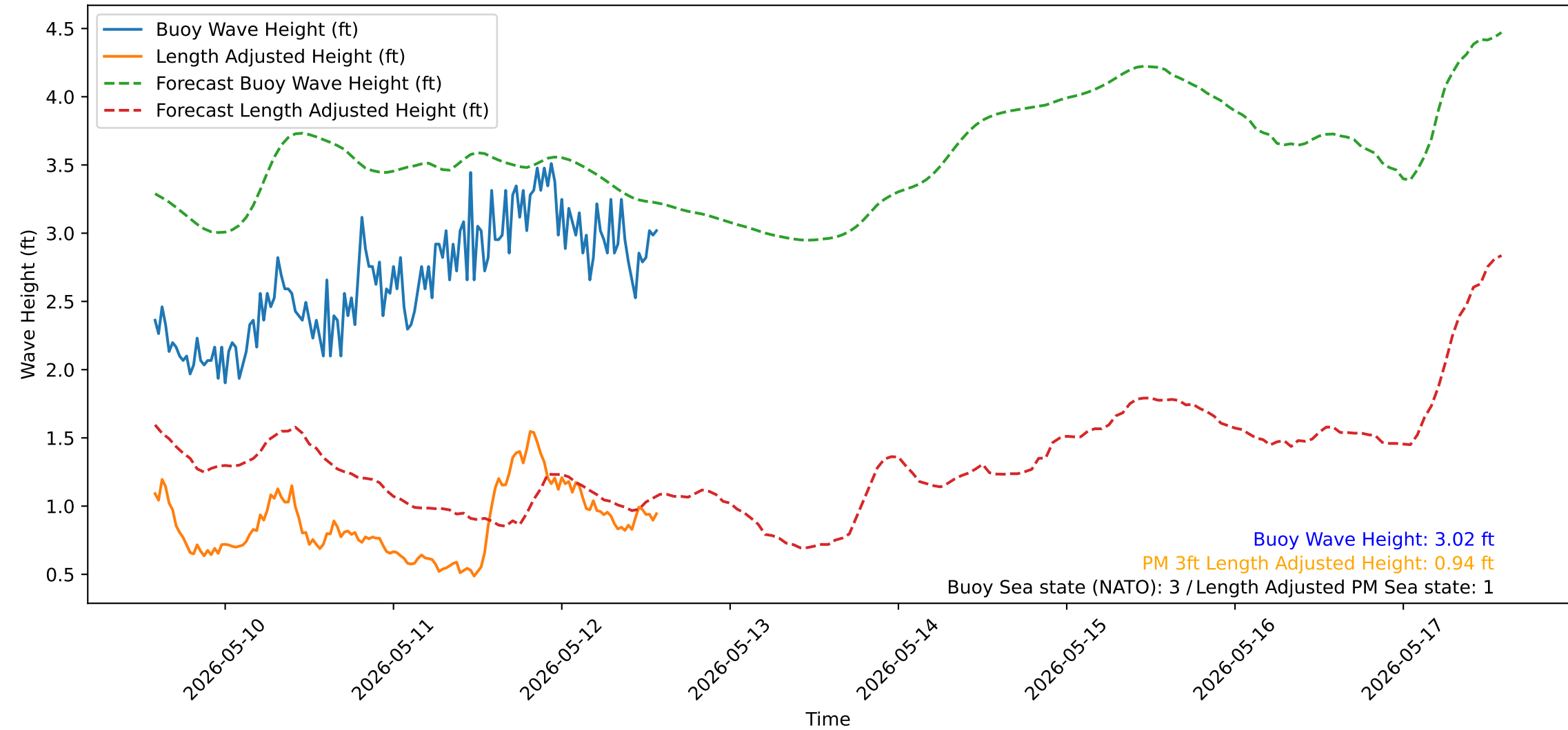
Wave Heights over Time for Green Beach at 2026-05-12 14:11:14
