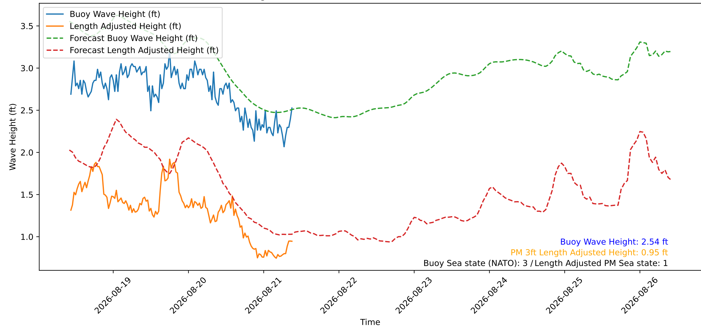
Wave Heights over Time for Red Beach at 2026-08-21 10:00:46
