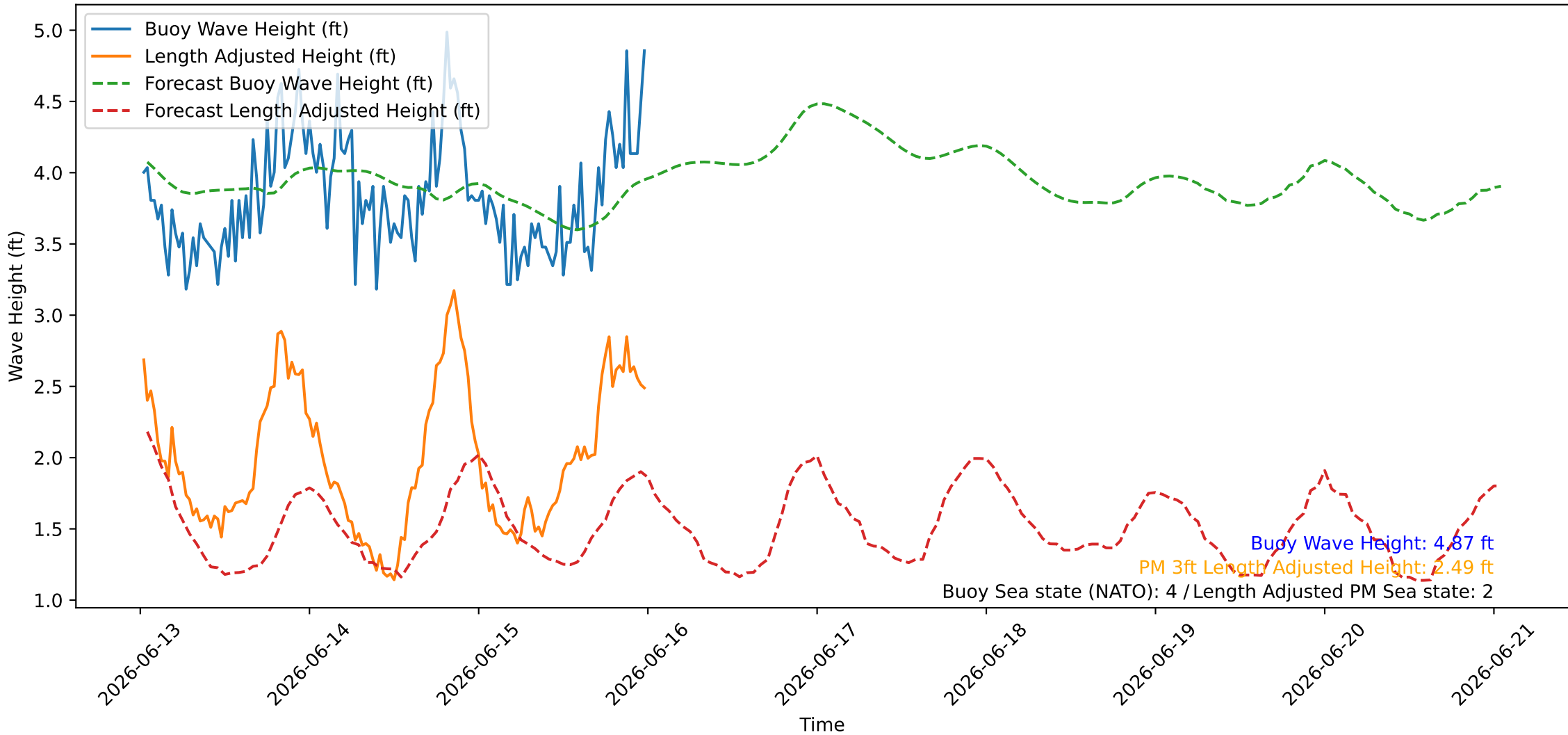
Wave Heights over Time for Oceanside Harbor at 2026-06-16 00:30:25
