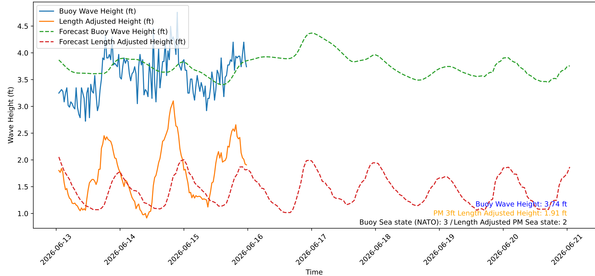
Wave Heights over Time for Red Beach at 2026-06-16 00:30:44
