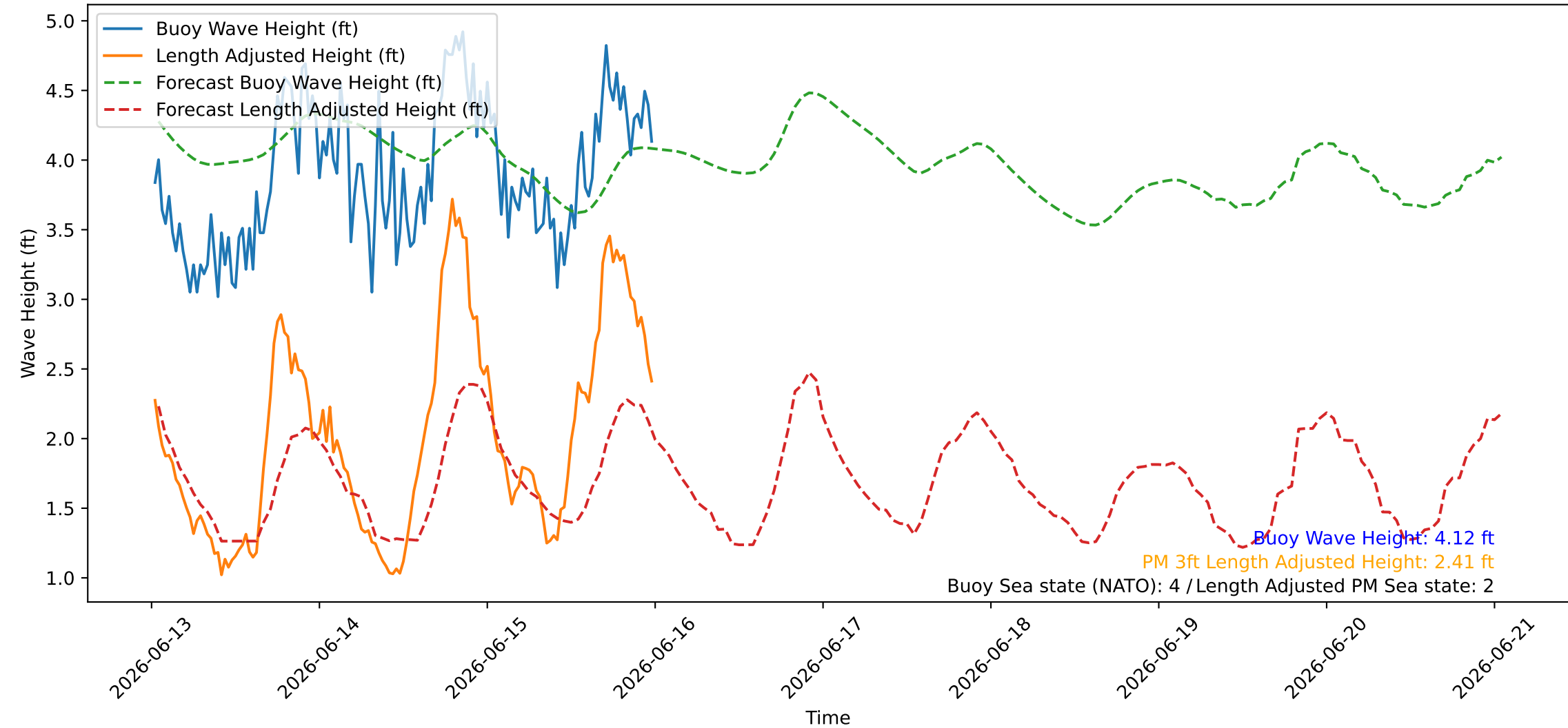
Wave Heights over Time for Green Beach at 2026-06-16 00:31:07
