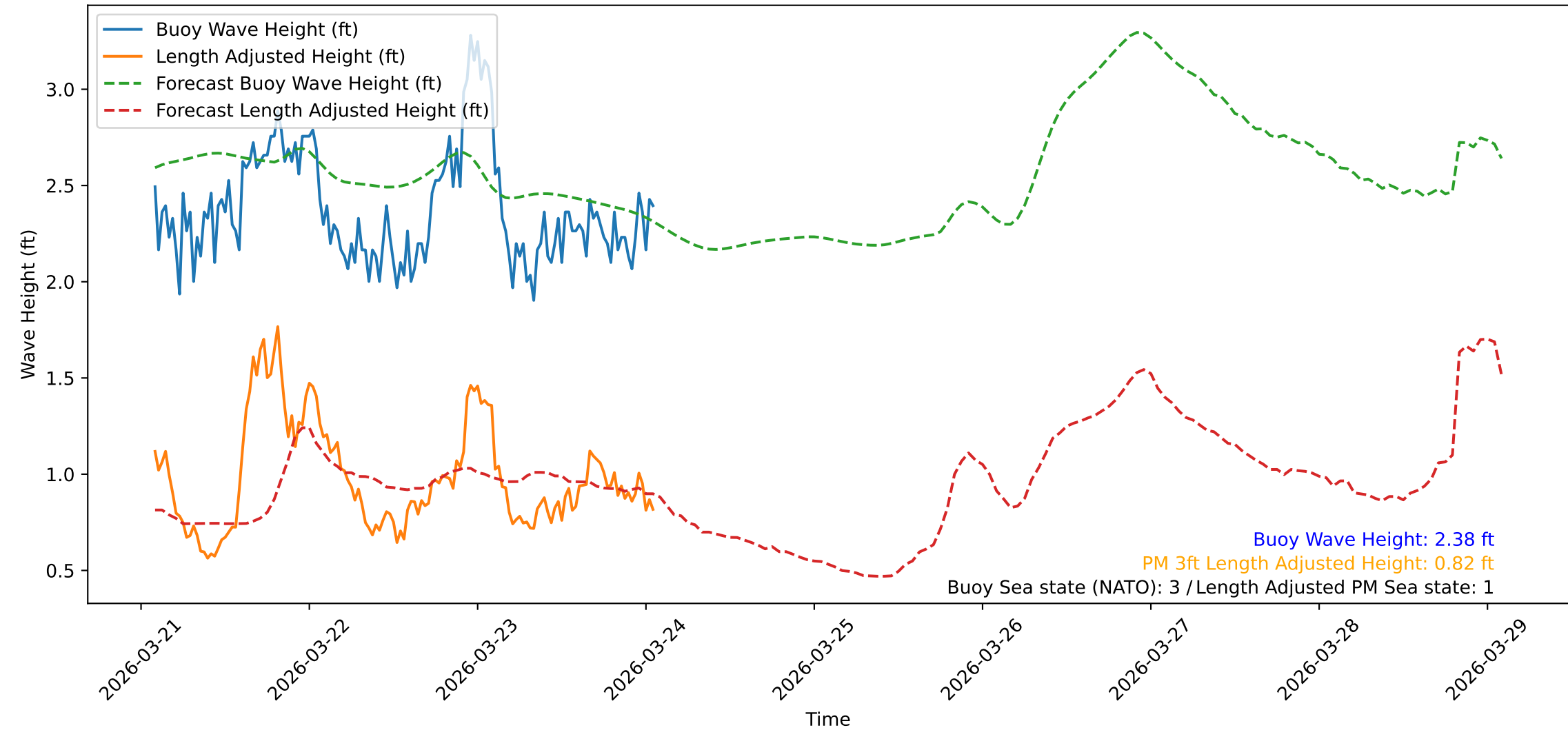
Wave Heights over Time for Green Beach at 2026-03-24 01:51:10
