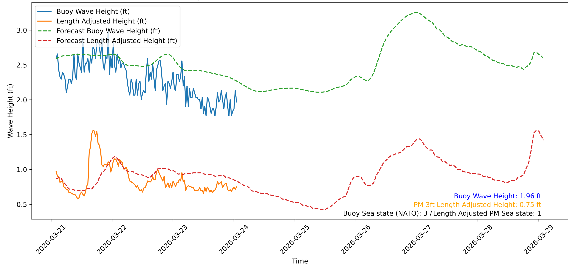
Wave Heights over Time for Oceanside Harbor at 2026-03-24 01:50:31
