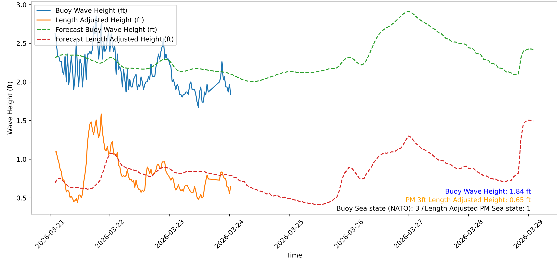
Wave Heights over Time for Red Beach at 2026-03-24 01:50:47
