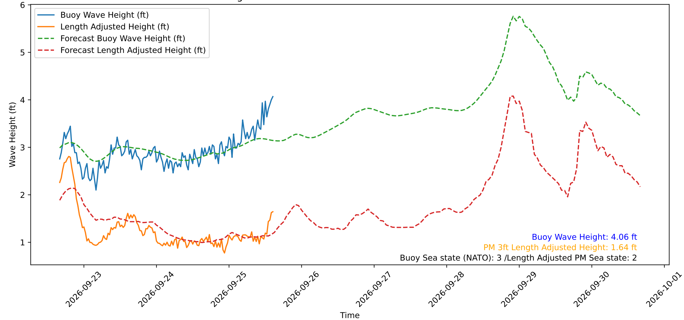
Wave Heights over Time for Green Beach at 2026-09-25 15:31:11
