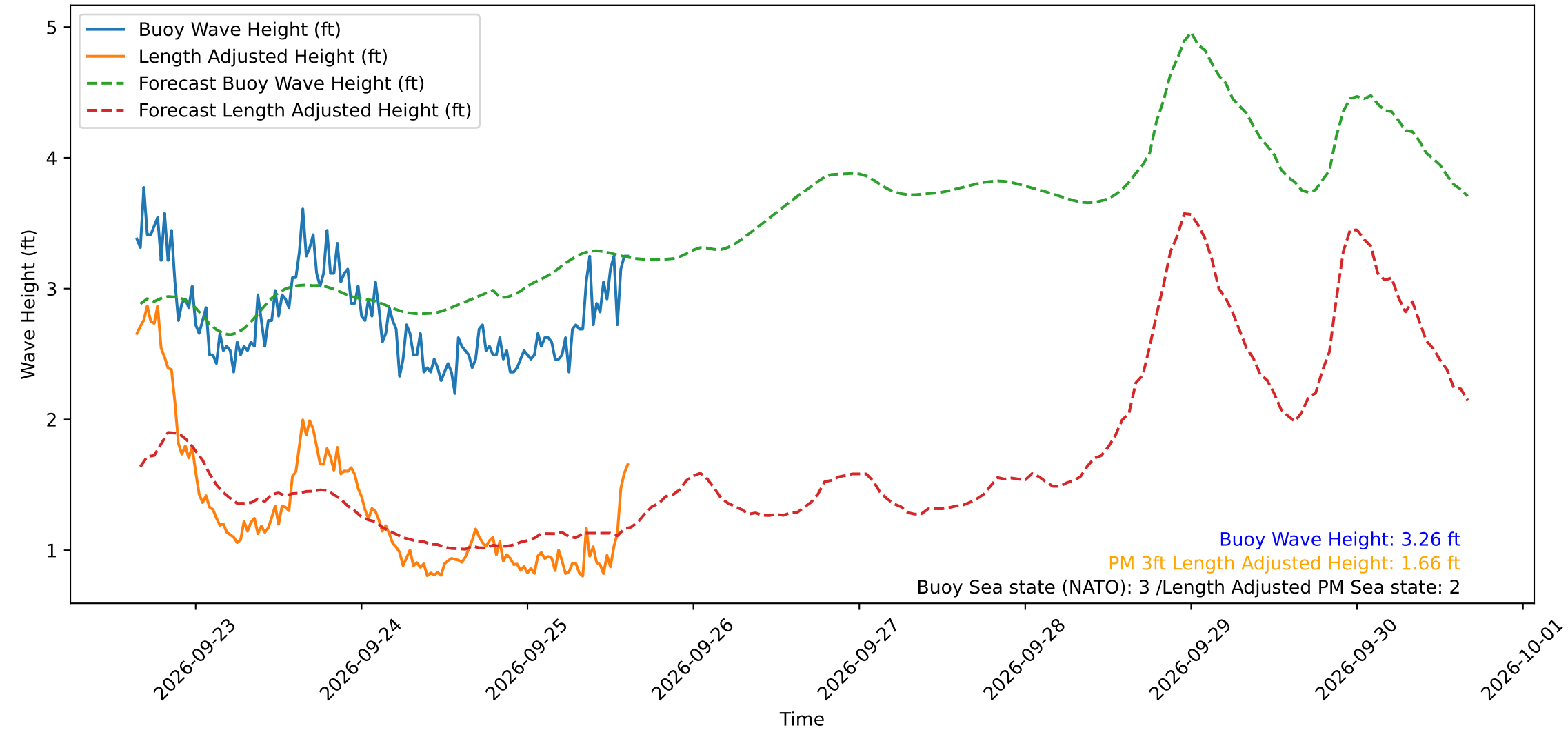
Wave Heights over Time for Oceanside Harbor at 2026-09-25 15:30:30
