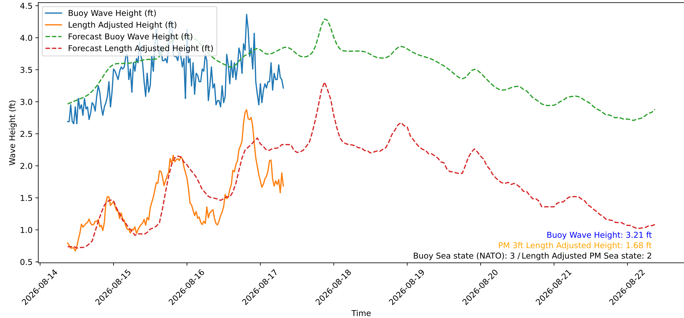
Wave Heights over Time for Green Beach at 2026-08-17 08:31:09
