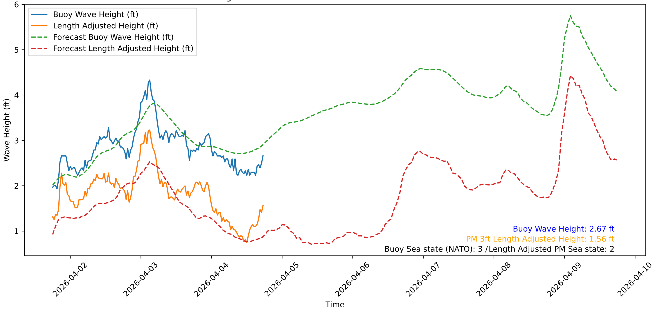
Wave Heights over Time for Green Beach at 2026-04-04 18:11:10
