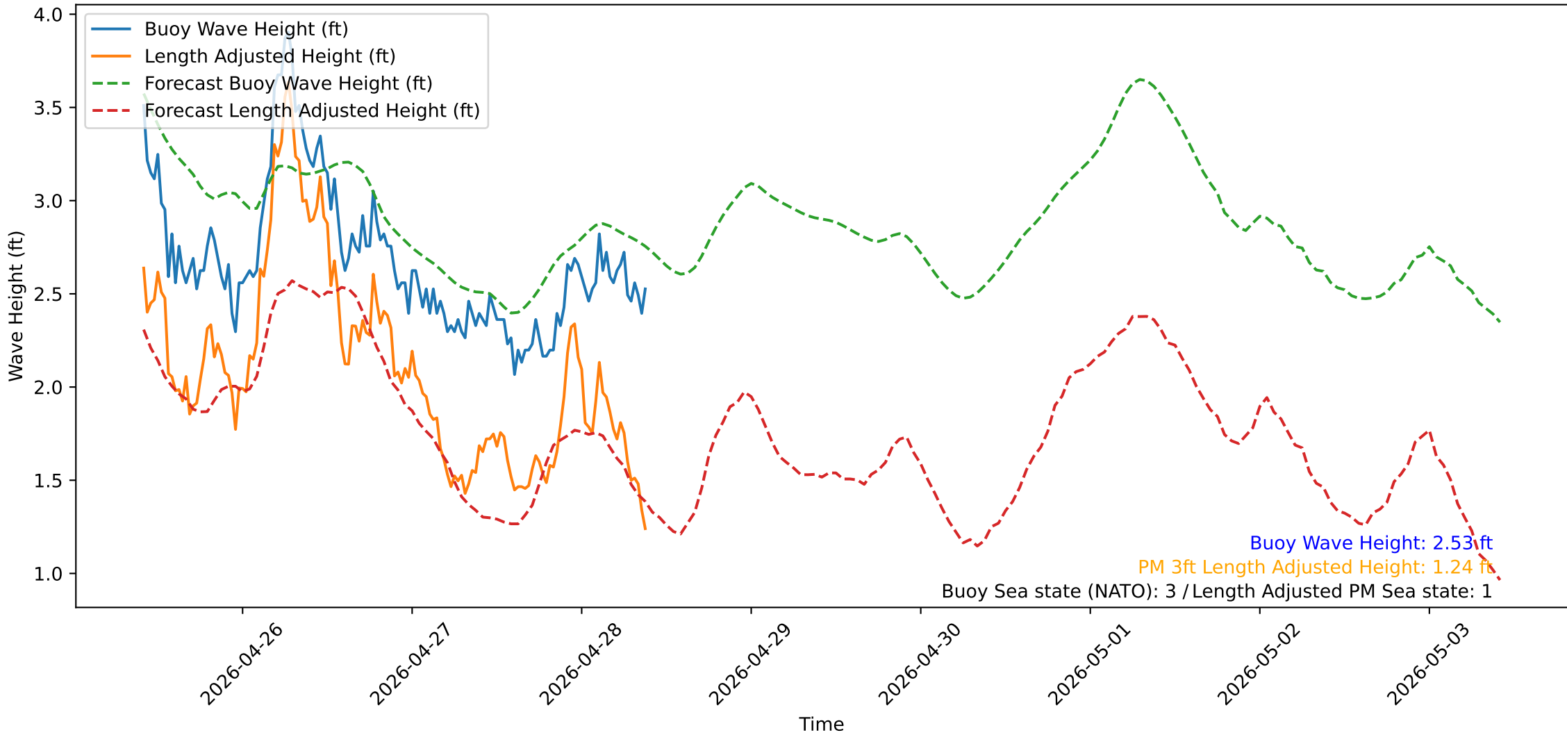
Wave Heights over Time for Oceanside Harbor at 2026-04-28 10:00:31
