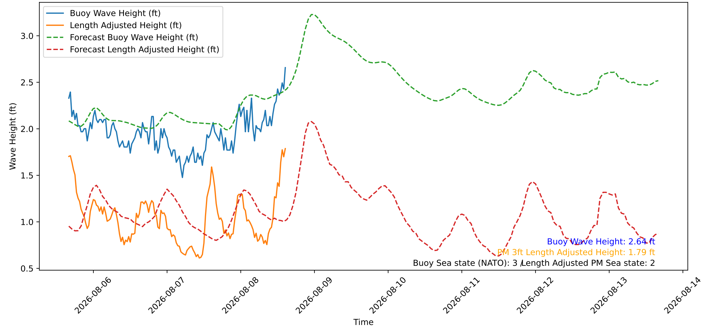
Wave Heights over Time for Red Beach at 2026-08-08 15:30:46
