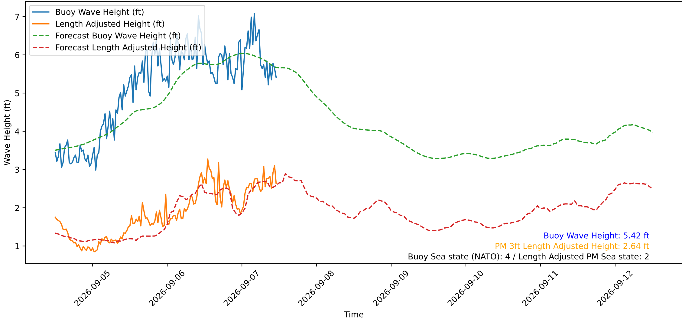
Wave Heights over Time for Oceanside Harbor at 2026-09-07 12:00:29
