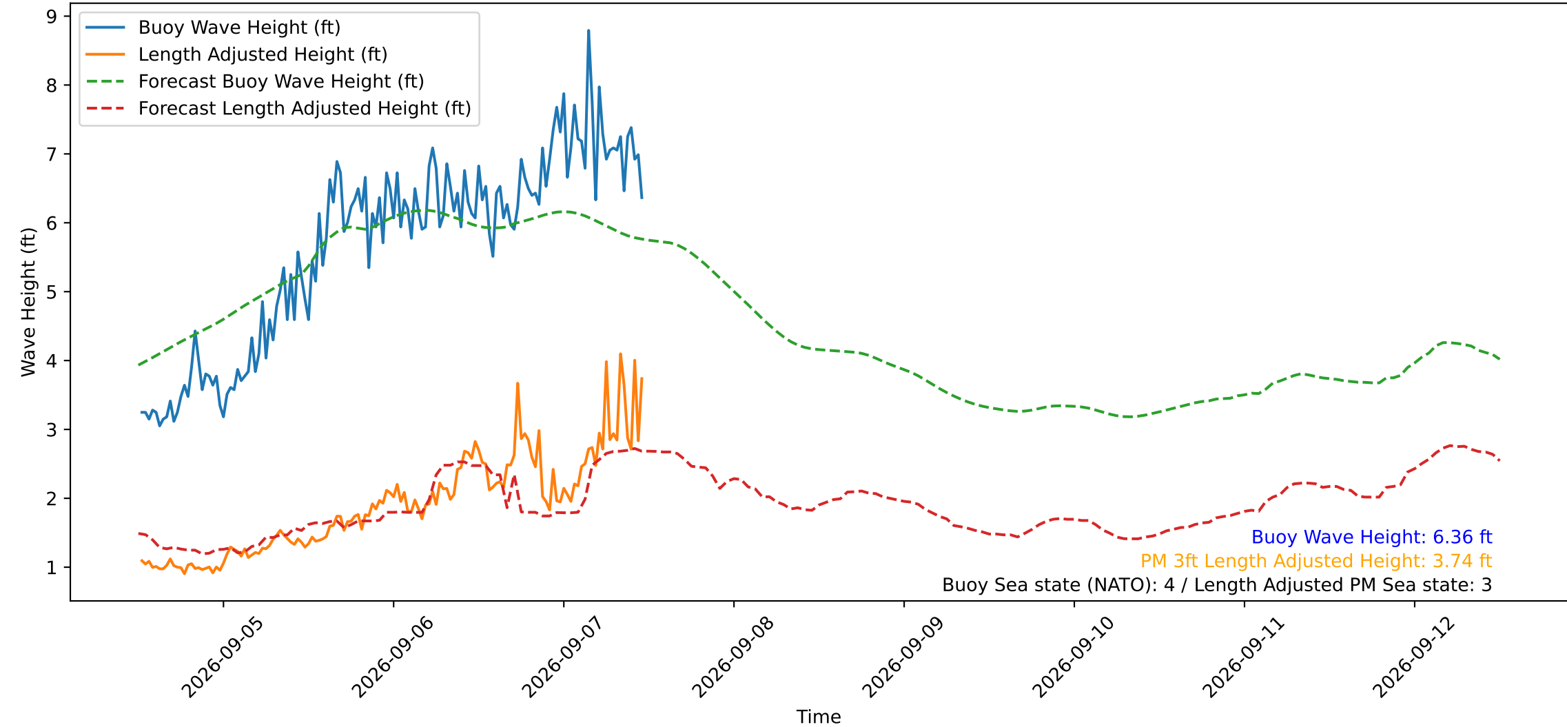
Wave Heights over Time for Green Beach at 2026-09-07 12:01:11
