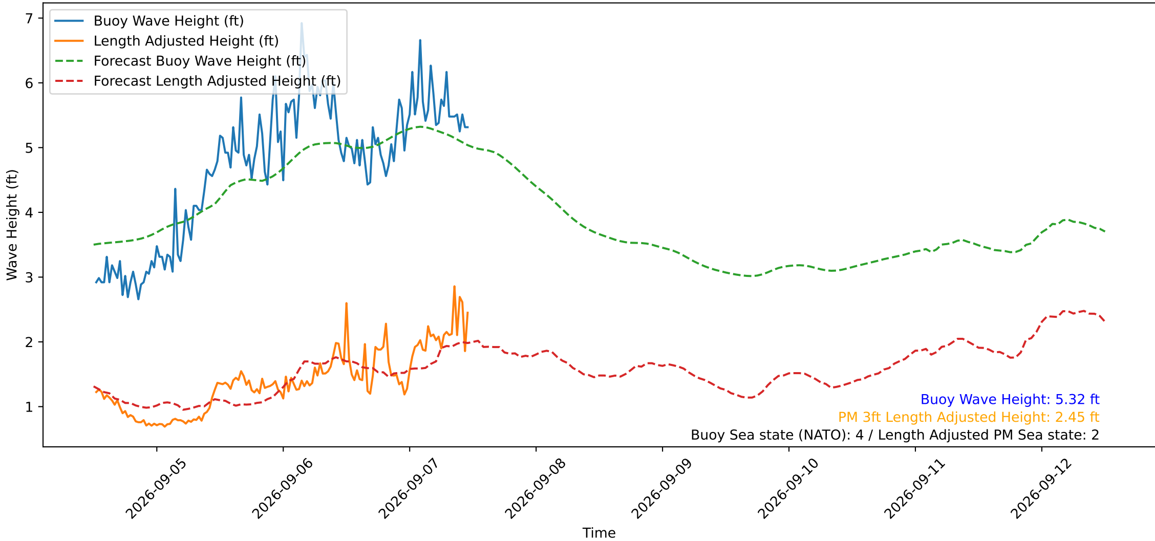
Wave Heights over Time for Red Beach at 2026-09-07 12:00:49
